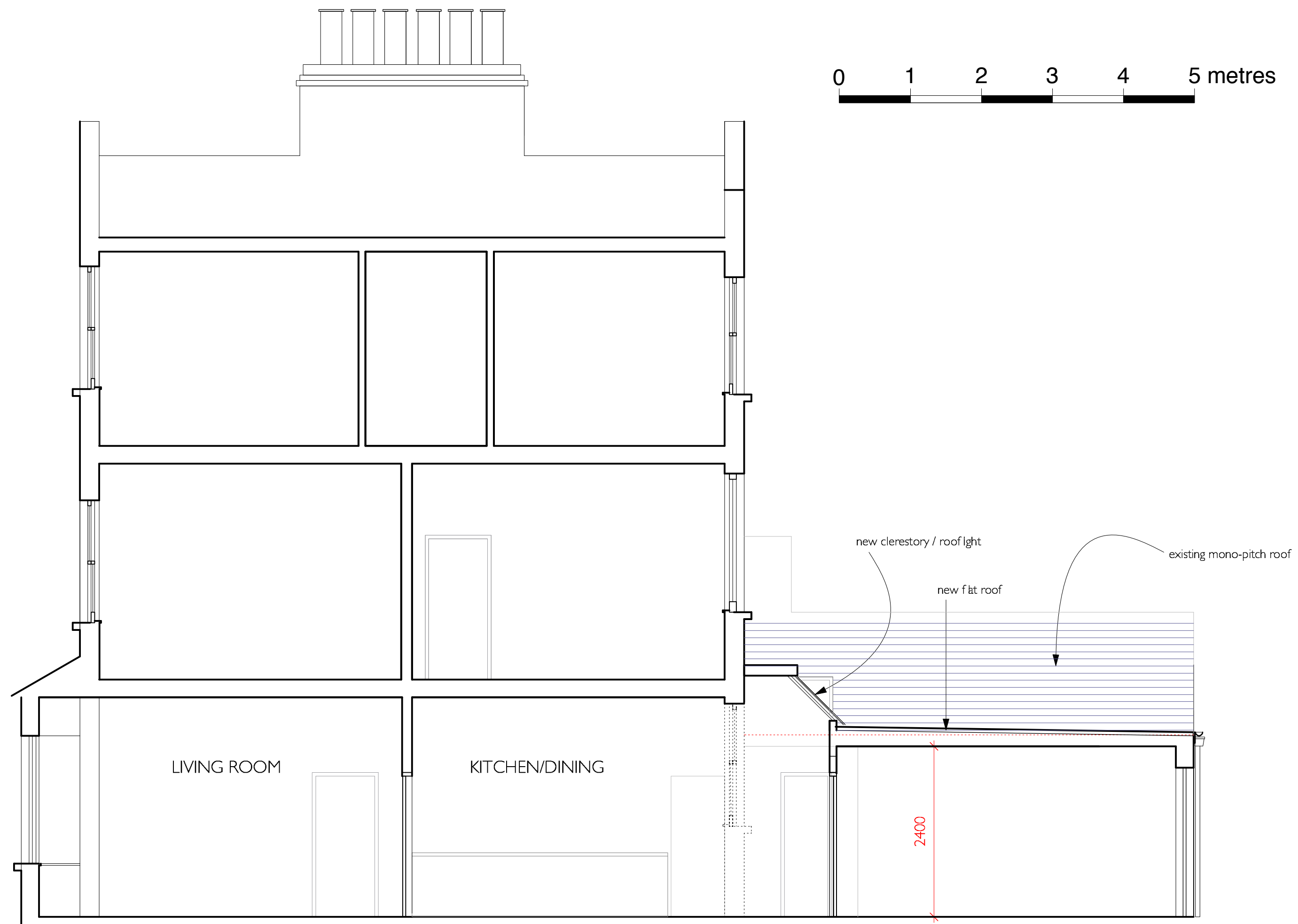
Section AA: As PROPOSED
