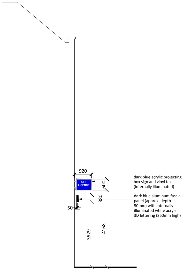
SIDE ELEVATION / TYPICAL SECTION PROPOSED
