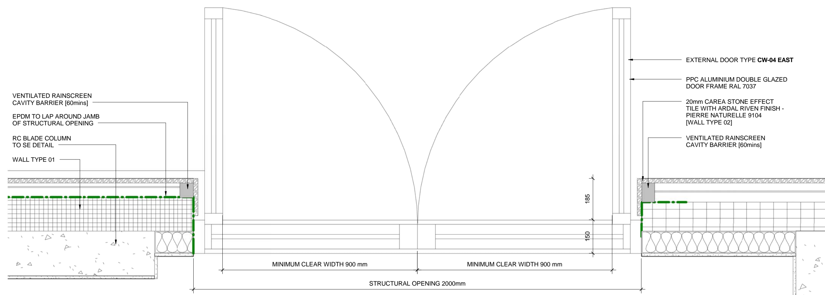
1 THRESHOLD DETAIL - COMMERCIAL DOOR - PLAN 1 : 10
