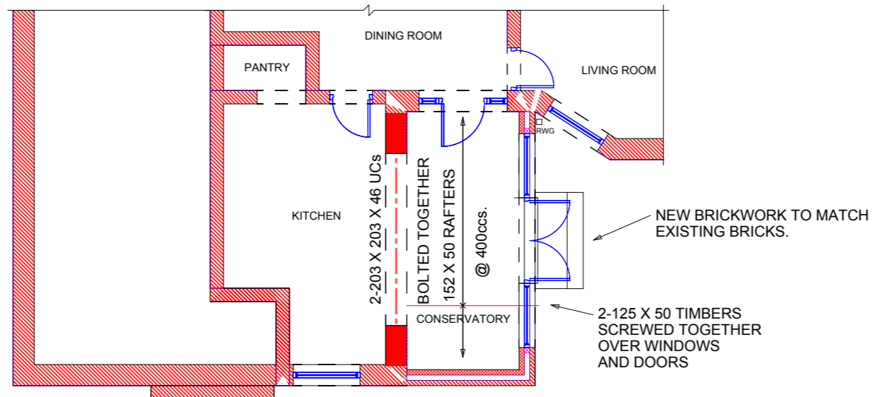
PROPOSED PART GROUND FLOOR PLAN
