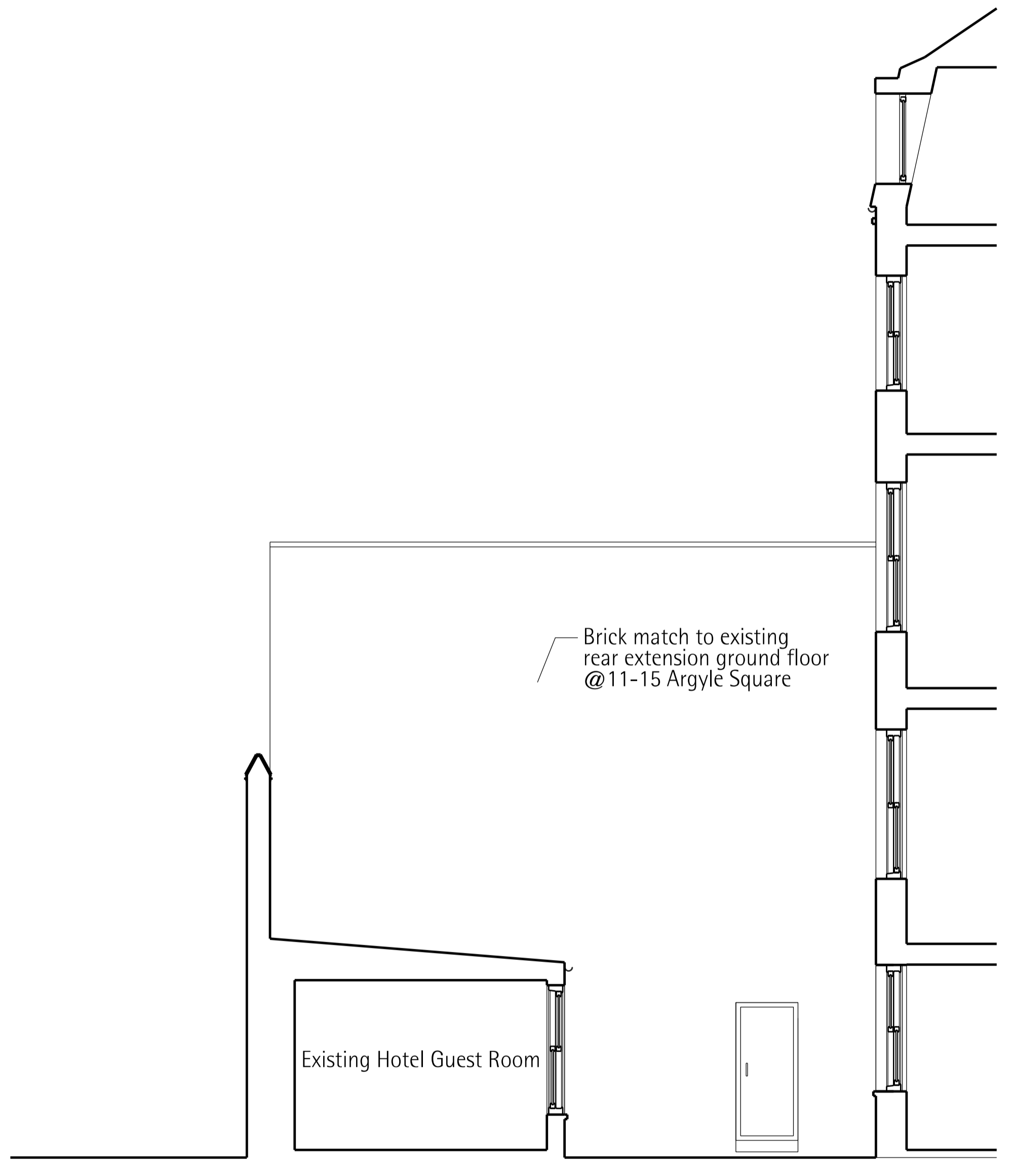
2. Proposed section C-C' Scale 1:50@A1
