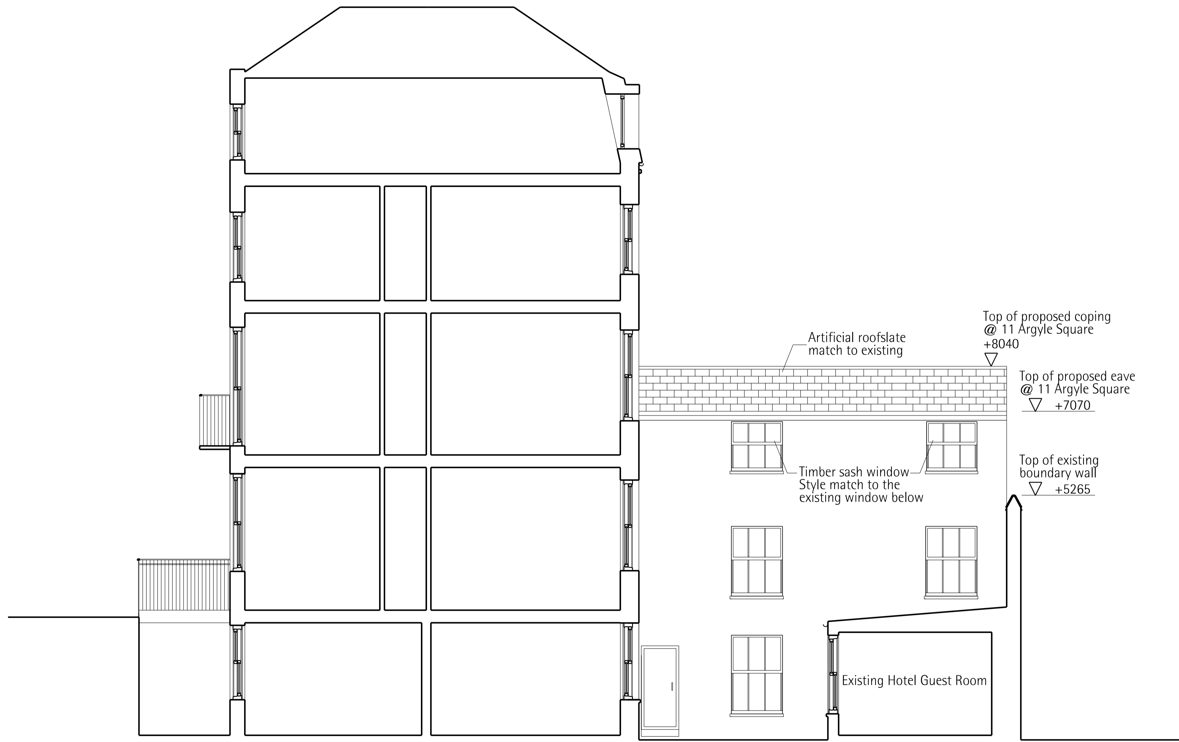
1. Proposed section B-B' Scale 1:50@A1
