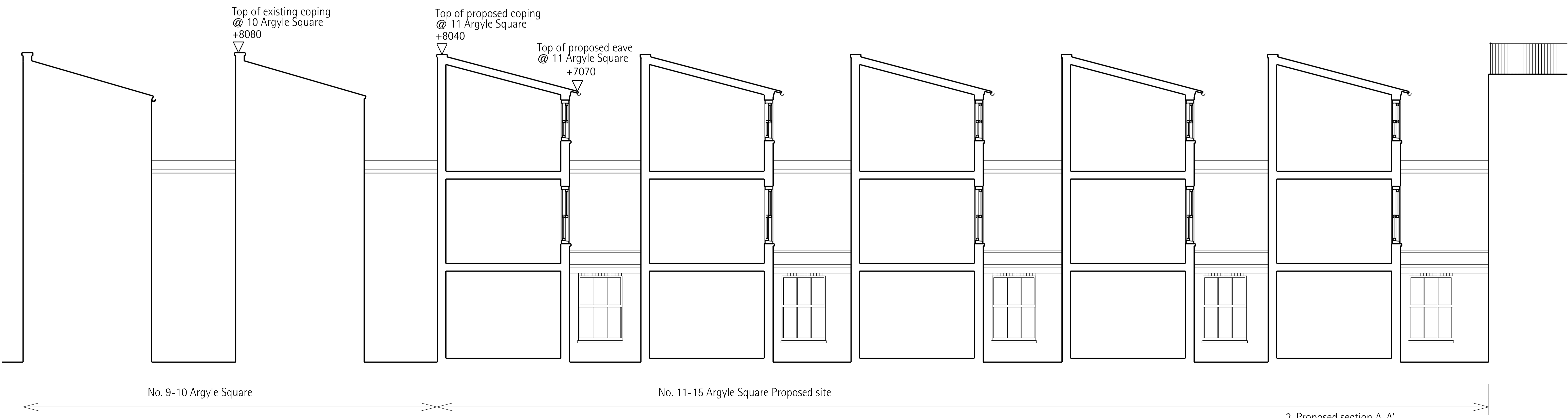
2. Proposed section A-A' Scale 1:50@A1
