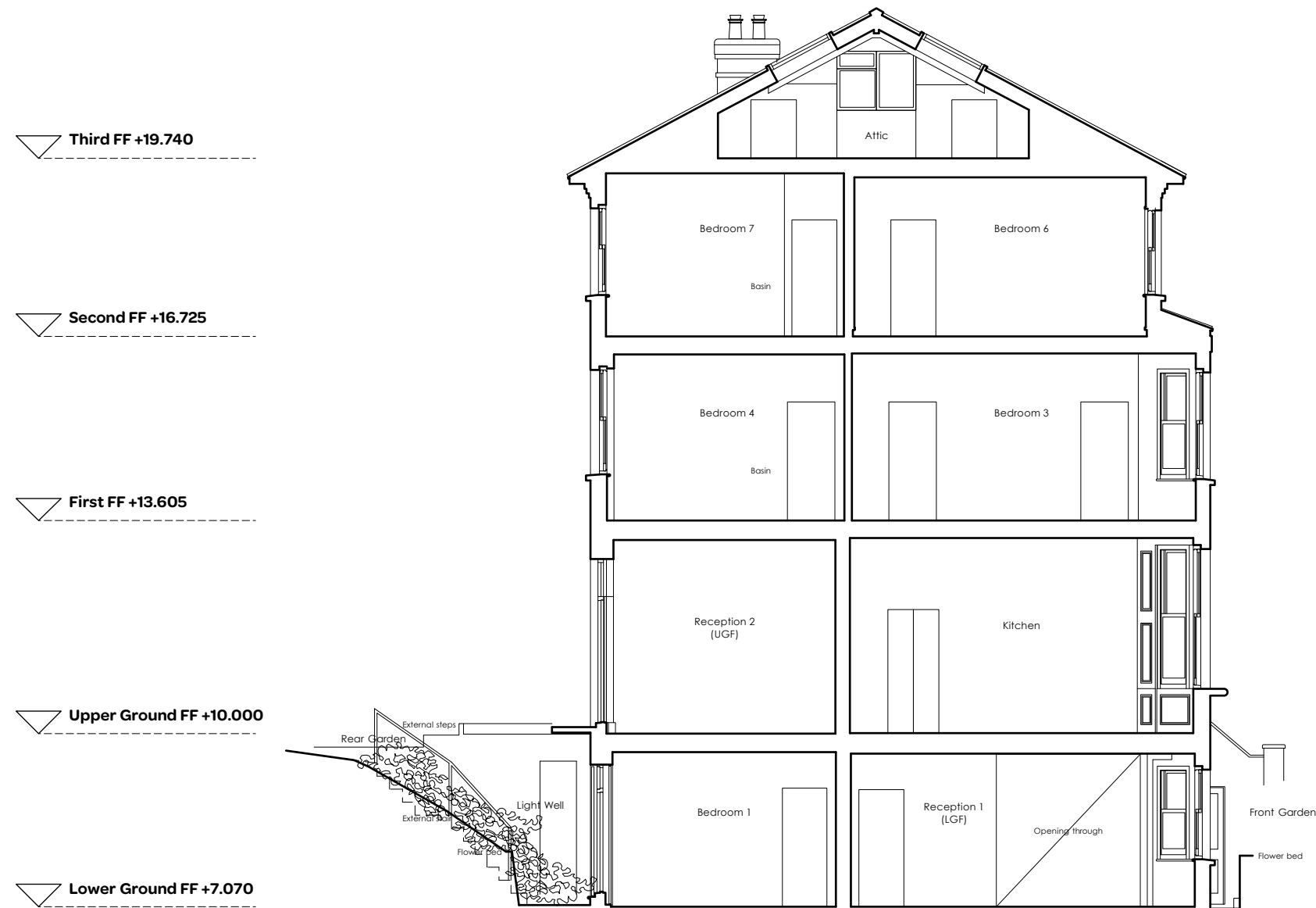
Existing Section
