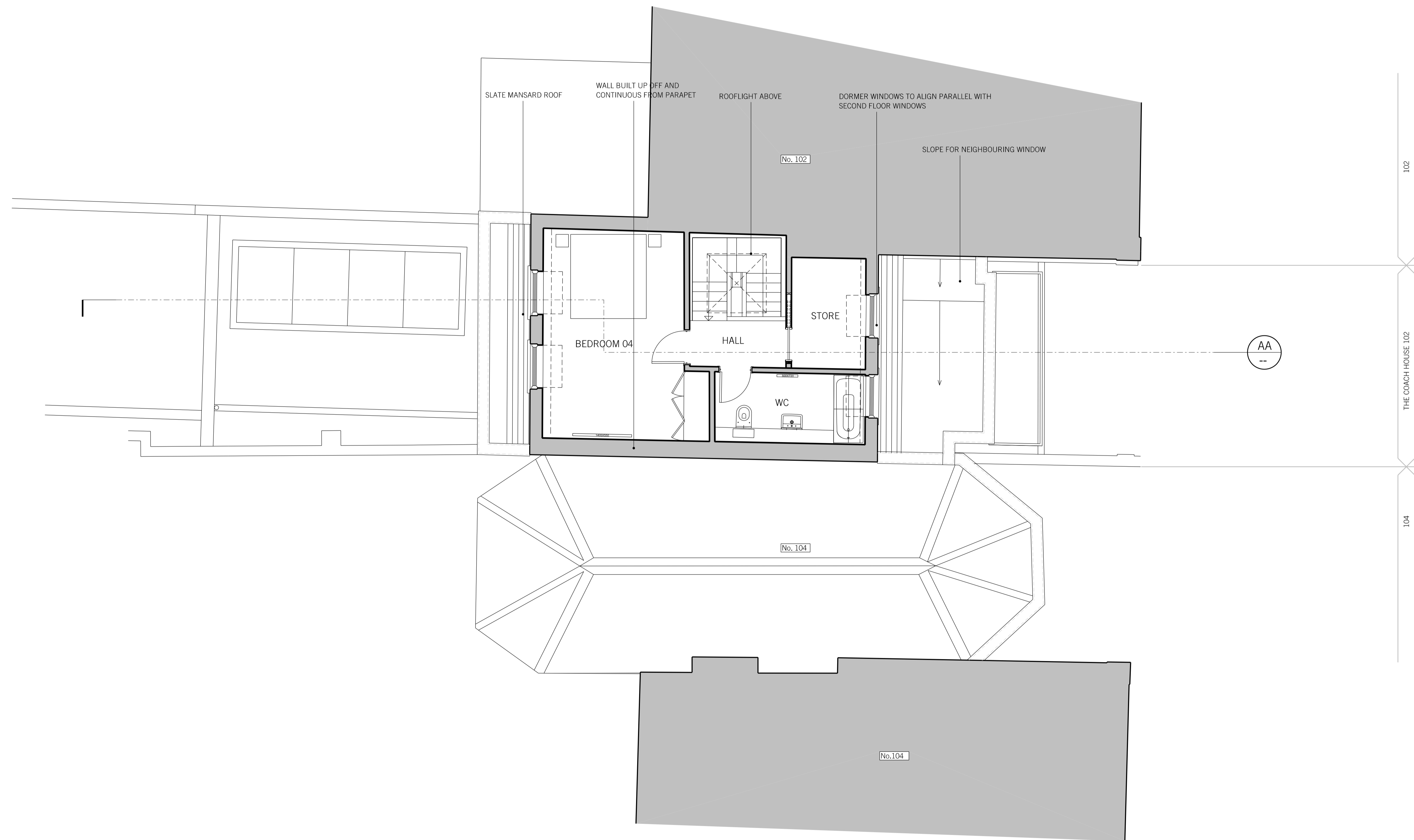
01: PROPOSED THIRD FLOOR PLAN SCALE 1:50
