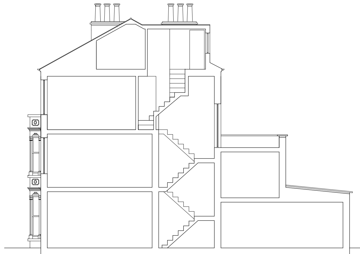
PROPOSED CROSS SECTION
