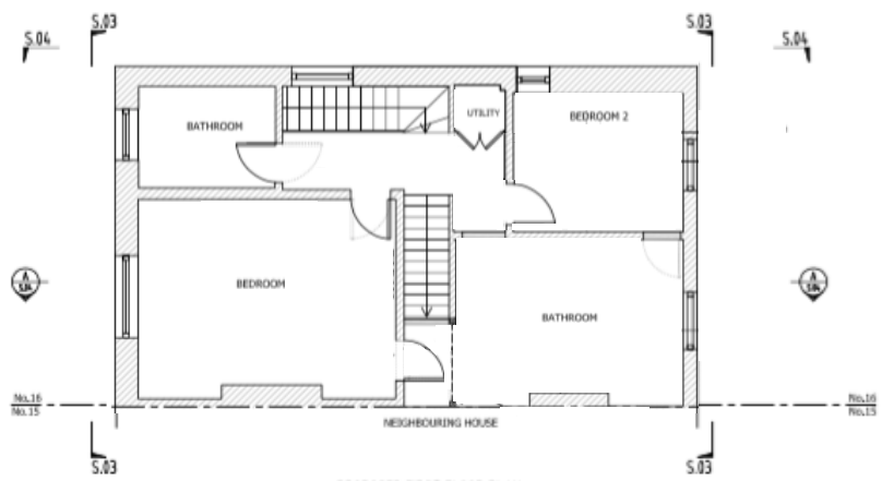
PROPOSED FIRST FLOOR PLAN SCALE 1/8" @ 1/4"
