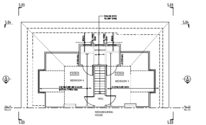
PROPOSED LOFT FLOOR PLAN SCALE 1/8" @ 1/4"
