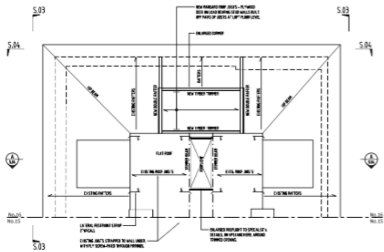
PROPOSED ROOF PLAN SCALE 1/8" @ 1/4"
