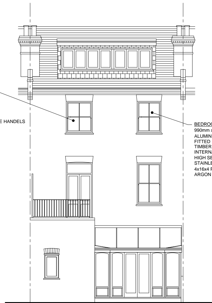
REAR ELEVATION
