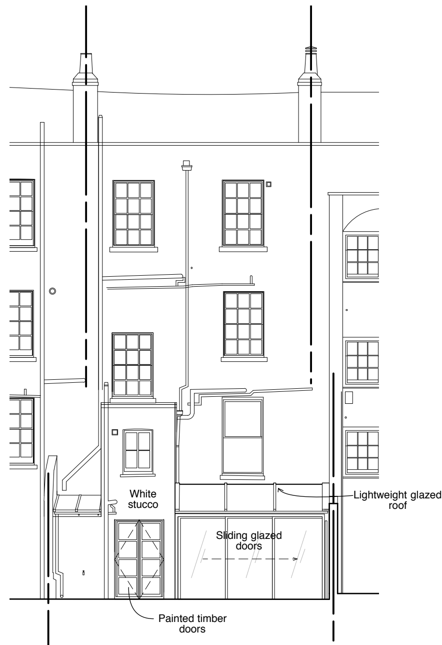
REAR ELEVATION
