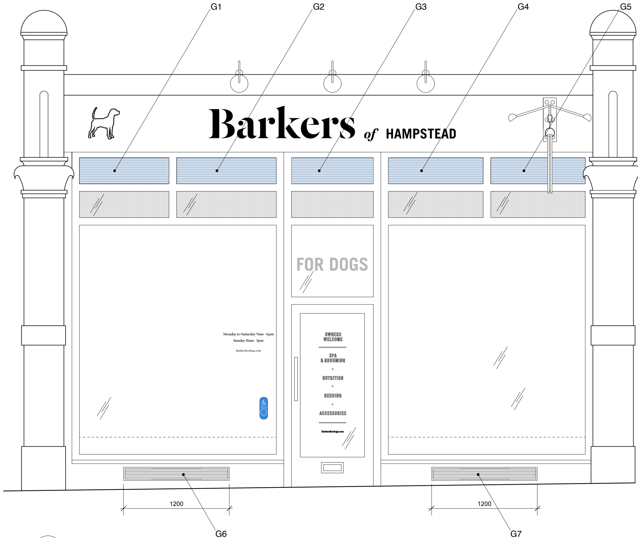
01 Shopfront Elevation 1:25@A3
