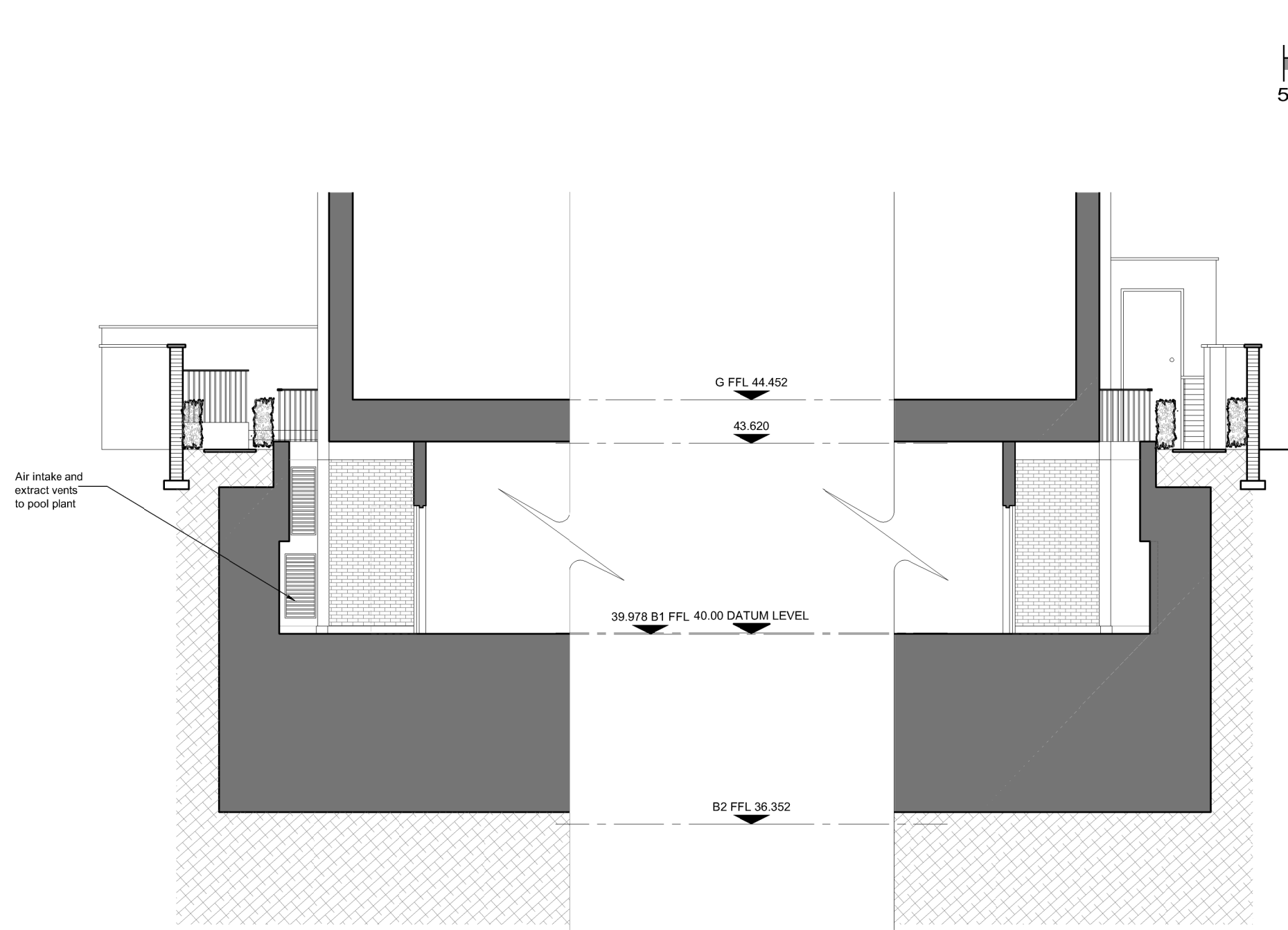
1 NORTH-WEST PARTIAL ELEVATION Scale: 1:50 CAD REF.
