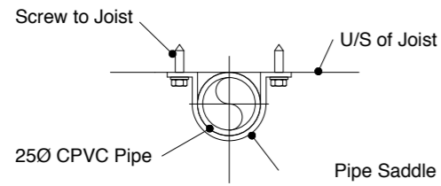
PROPOSED PIPE SUPPORT METHOD NOT TO SCALE
