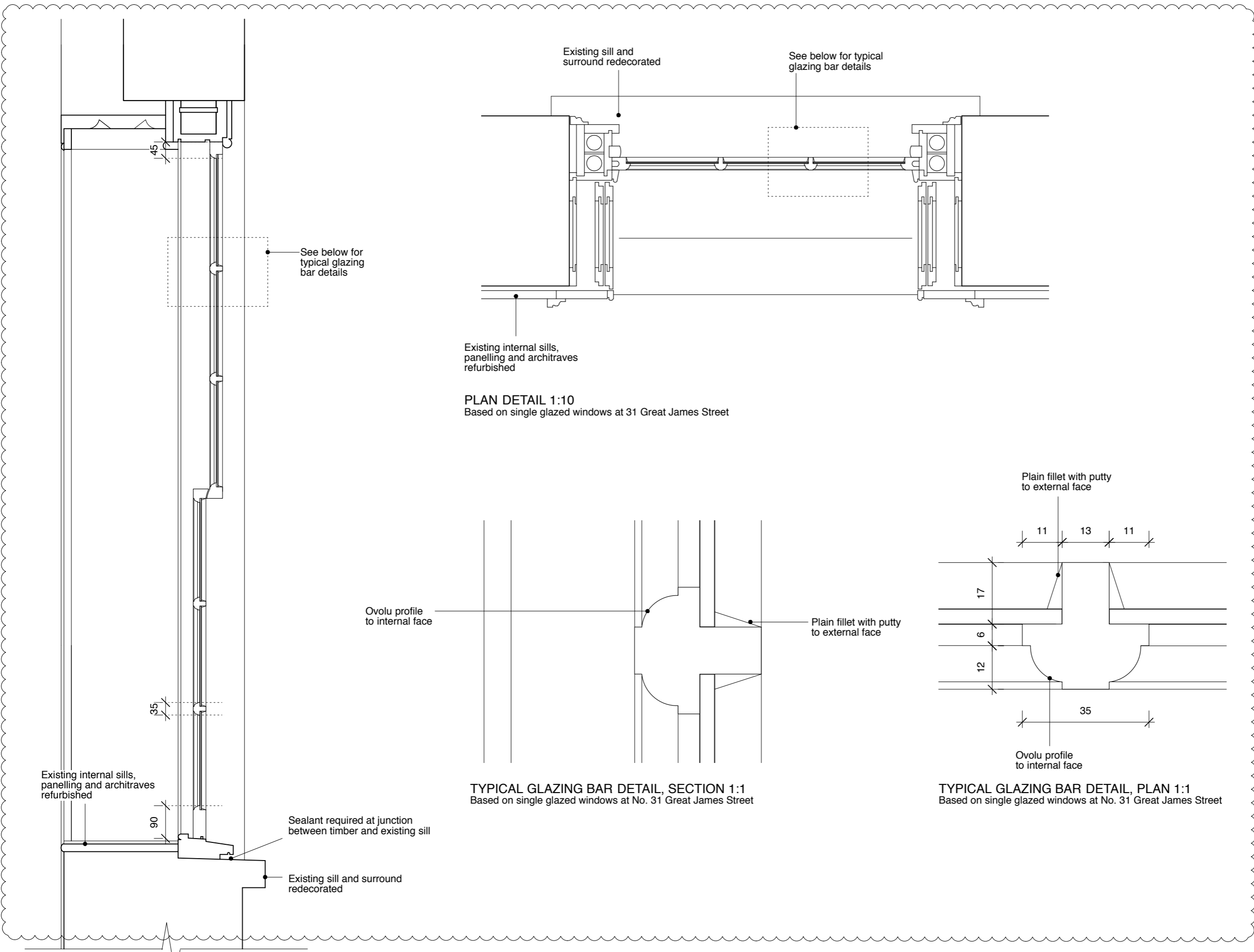
SECTION DETAIL 1:10 Based on single glazed windows at No. 31 Great James Street
