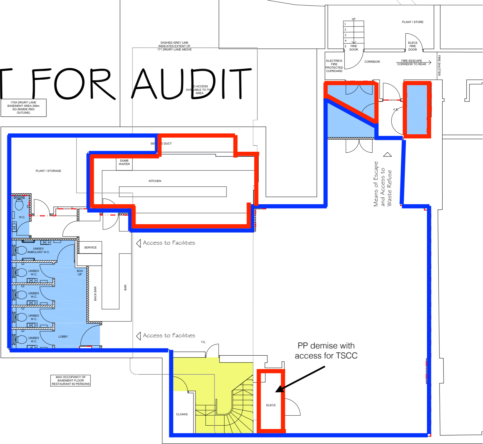
BASEMENT PLAN
