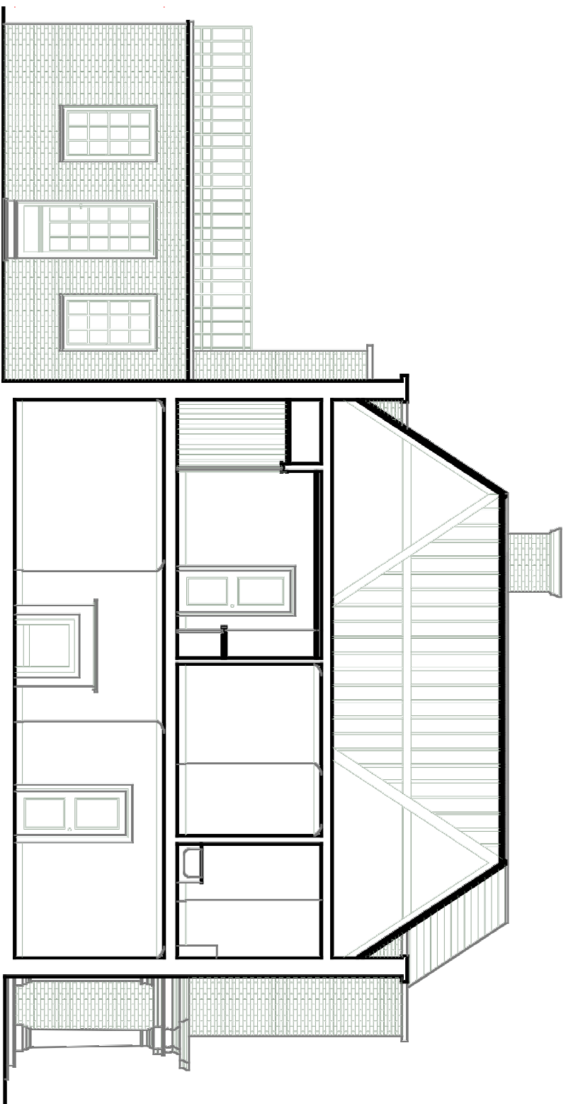
SECTION DD AS EXISTING
