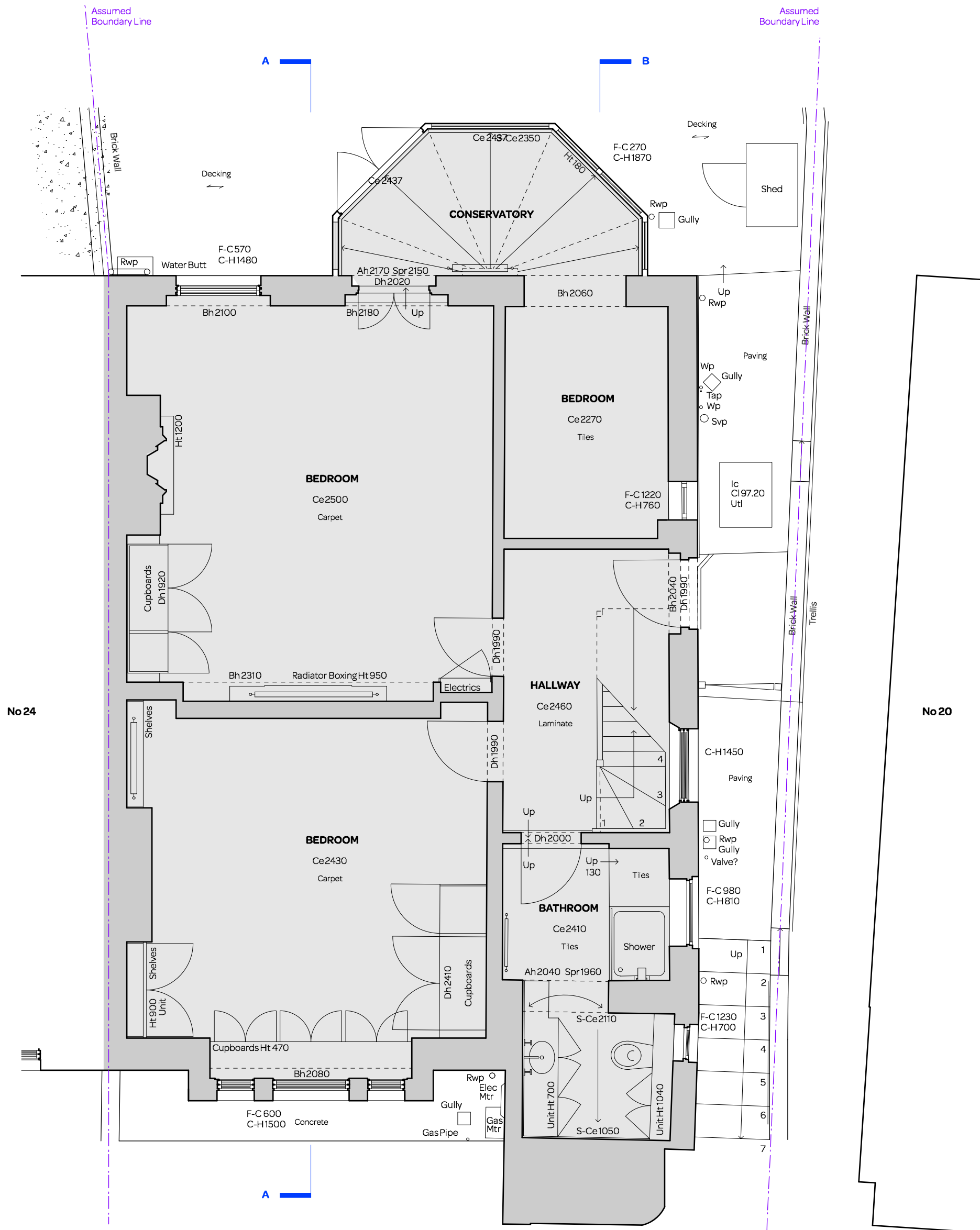
EXISTING LOWER GROUND FLOOR PLAN
