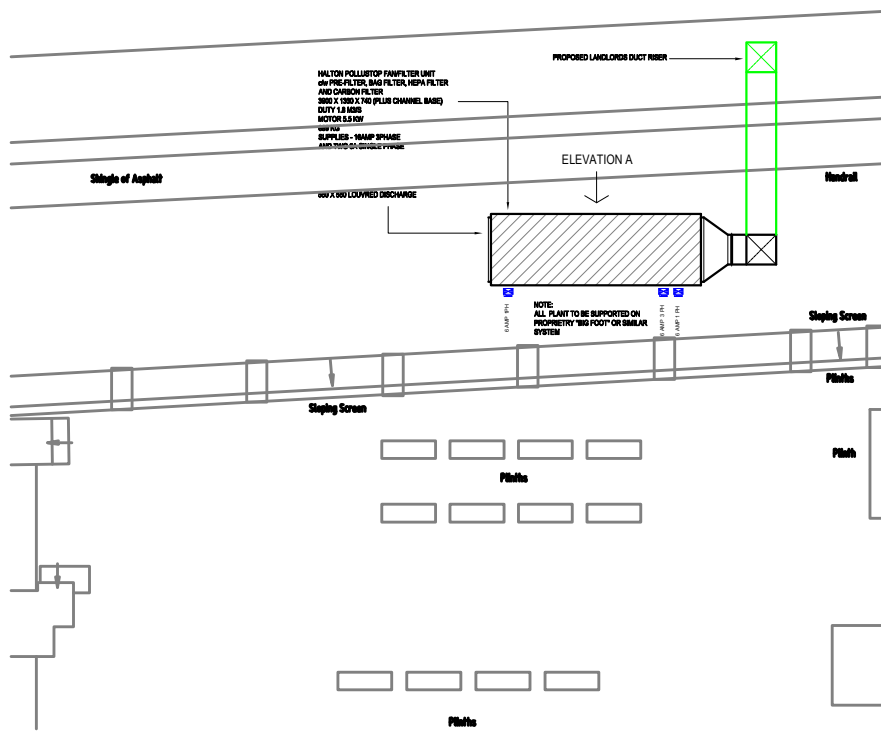
ENLARGED PLAN 1-50
