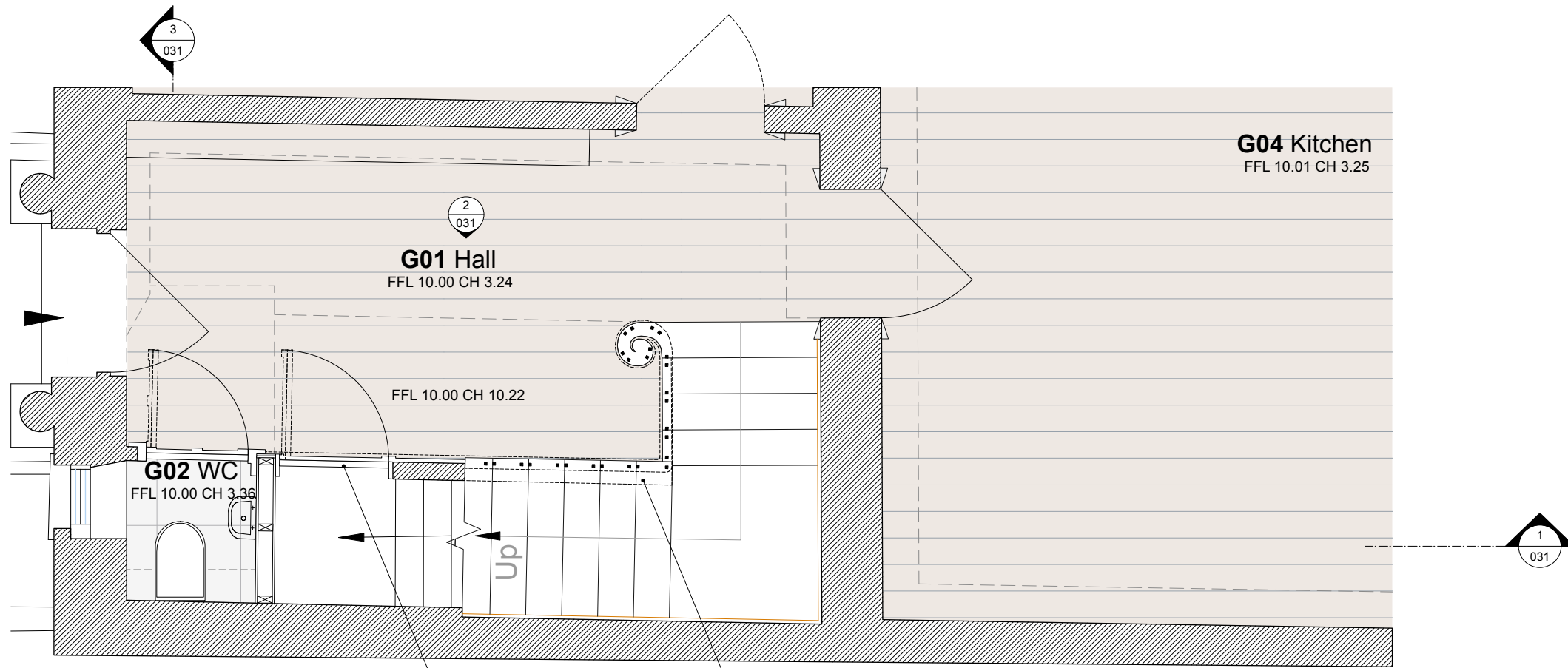
1 030 Proposed Stair Ground Floor Plan
