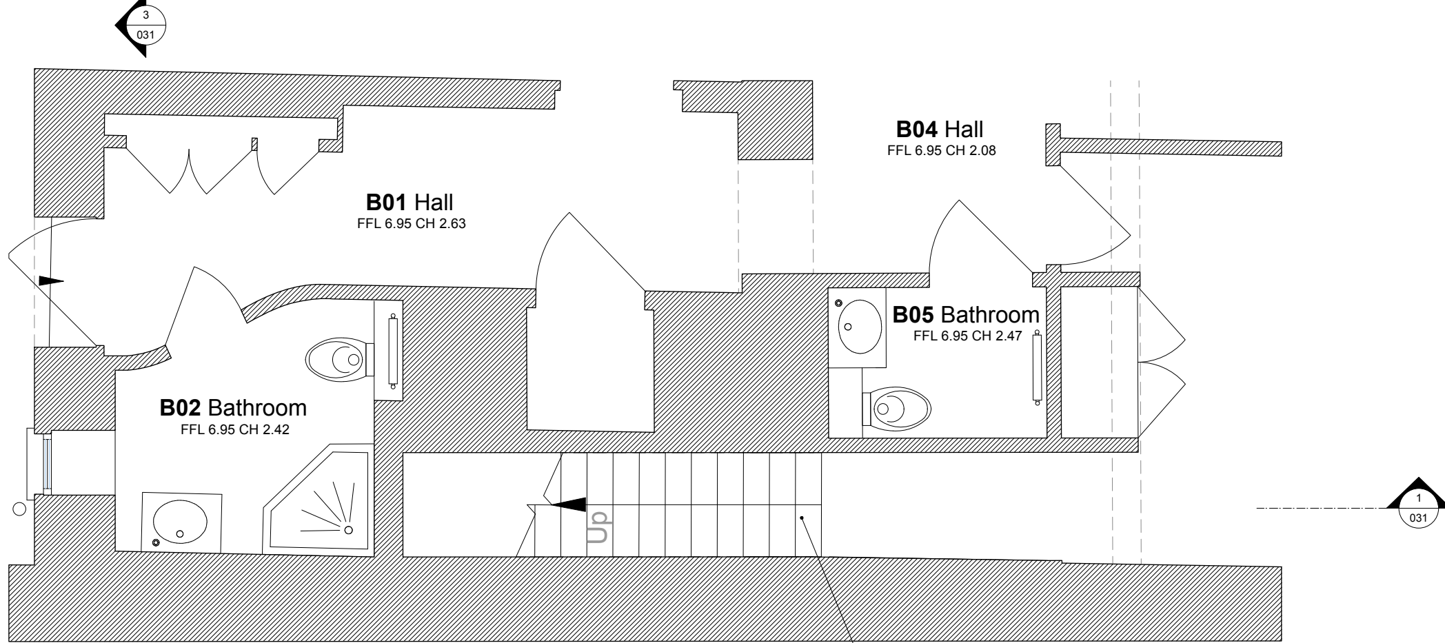
2 030 Proposed Stair Lower Ground Floor Plan
