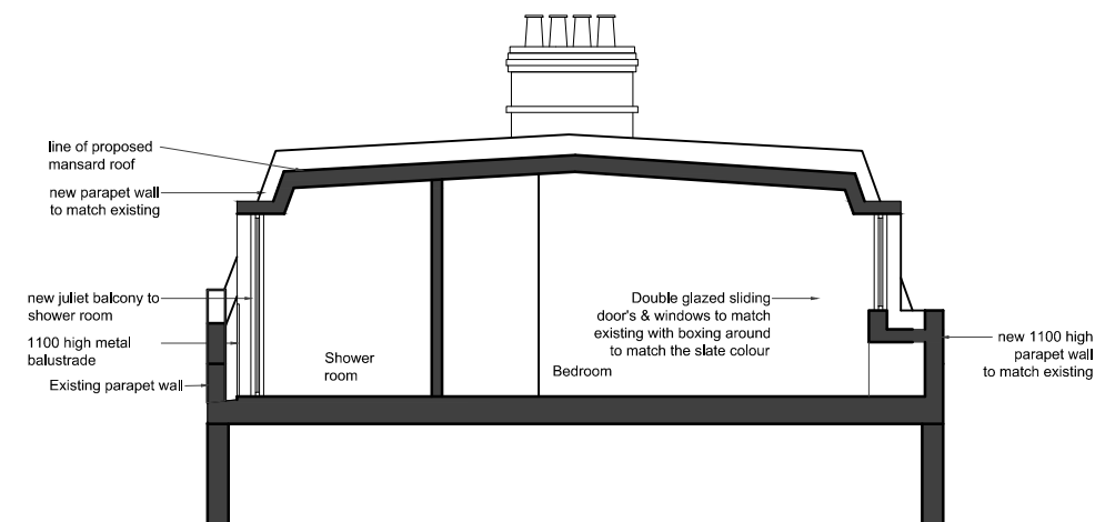
04- PART SECTION AA
