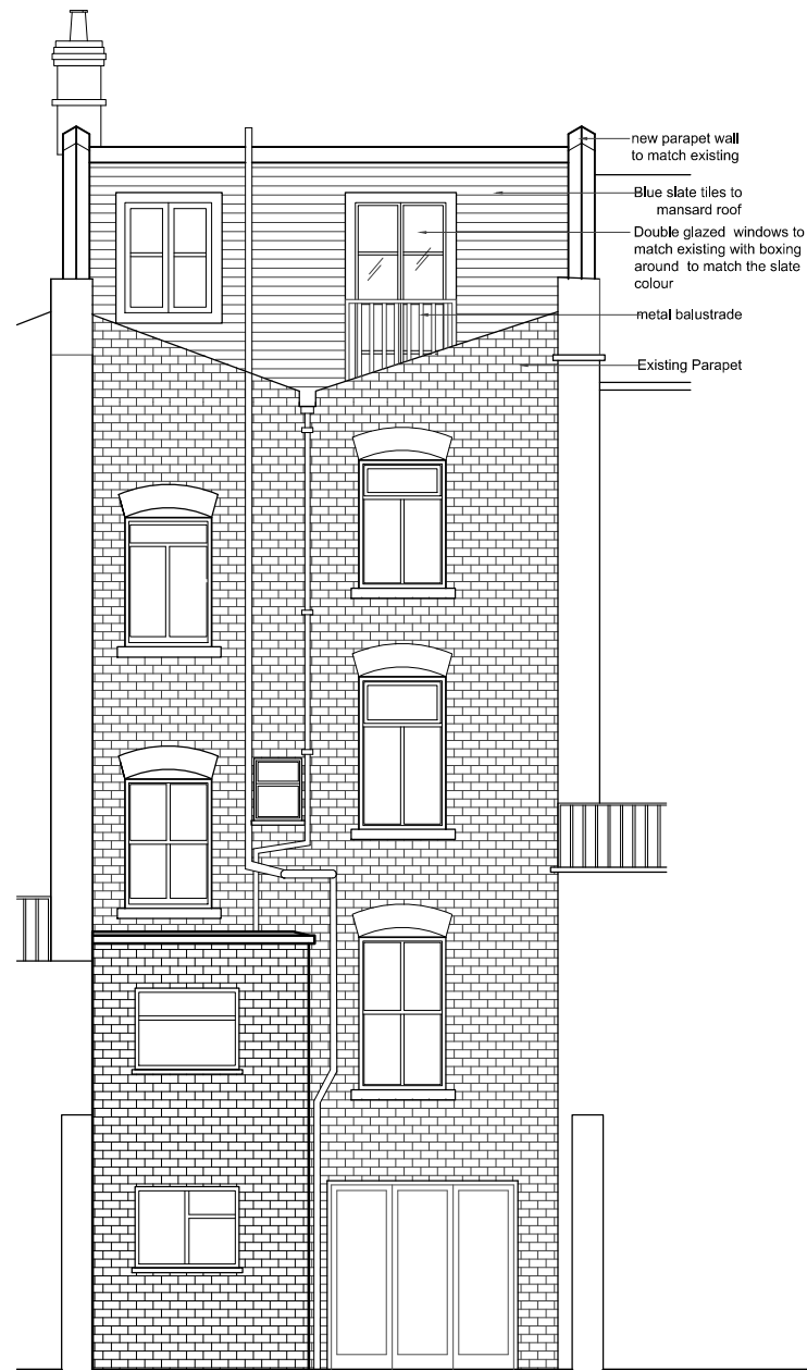
02- REAR ELEVATION
