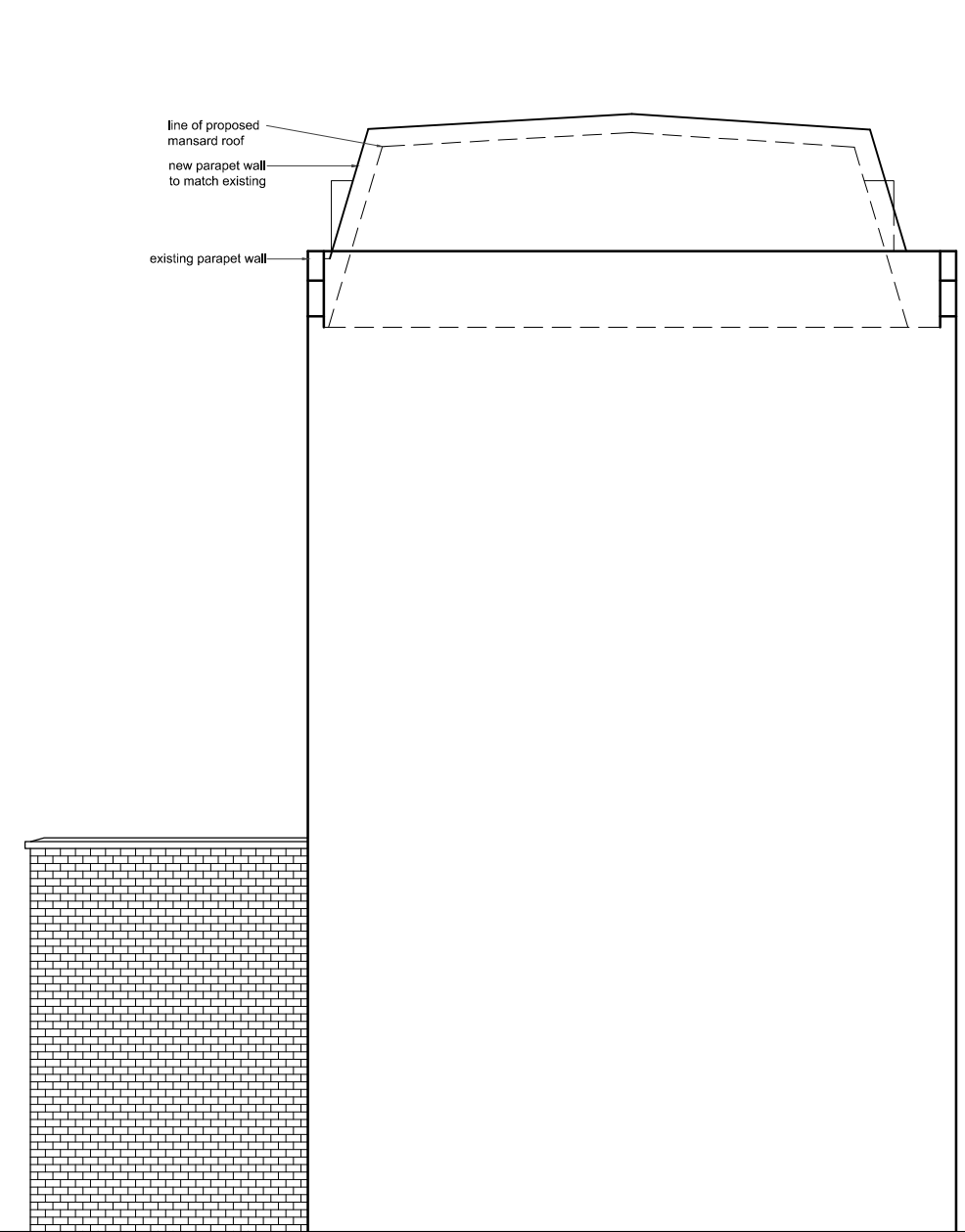
03- SIDE ELEVATION
