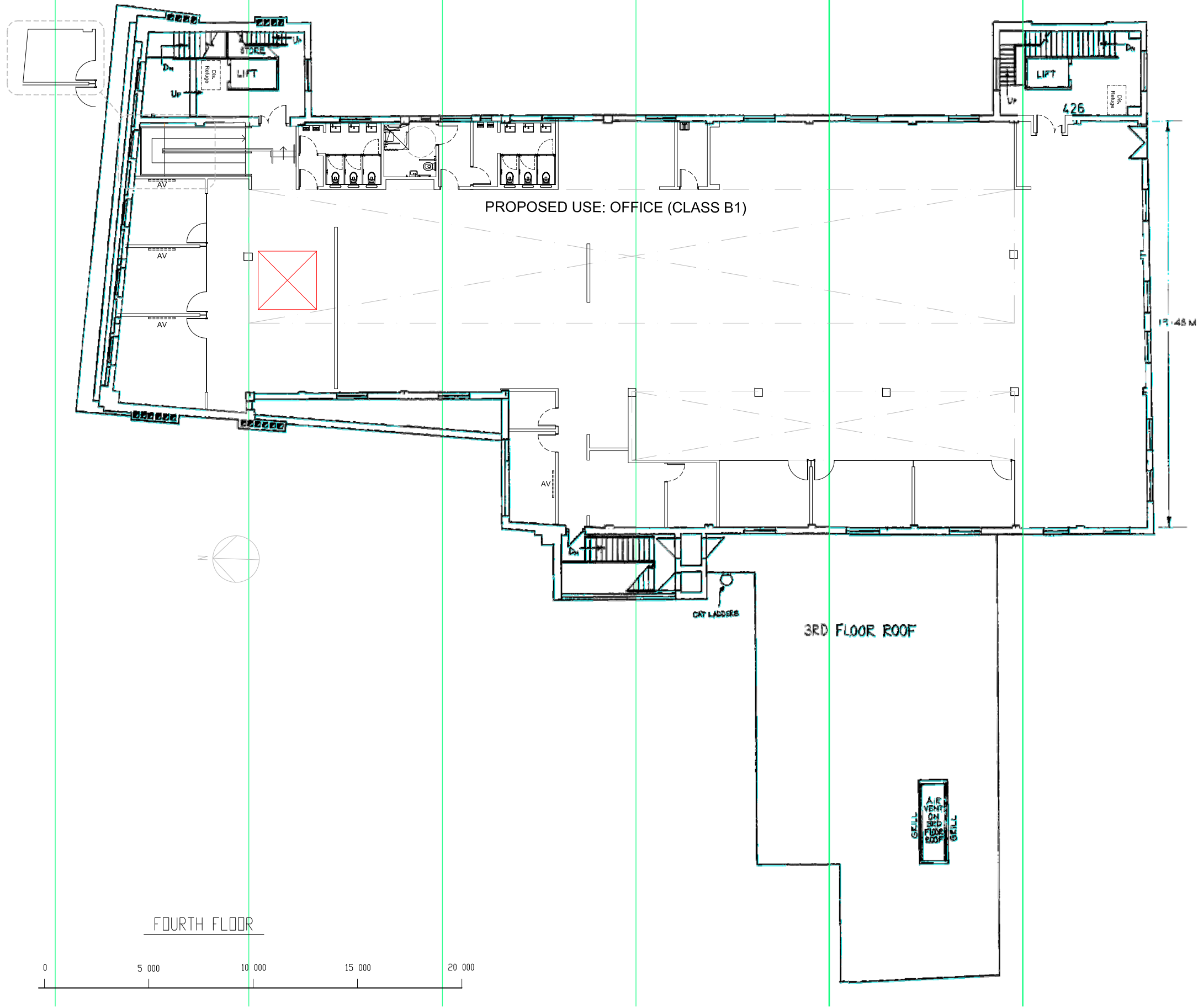
FOURTH FLOOR - GA PLAN PROPOSED 1:100@A1, 1:200@A3
