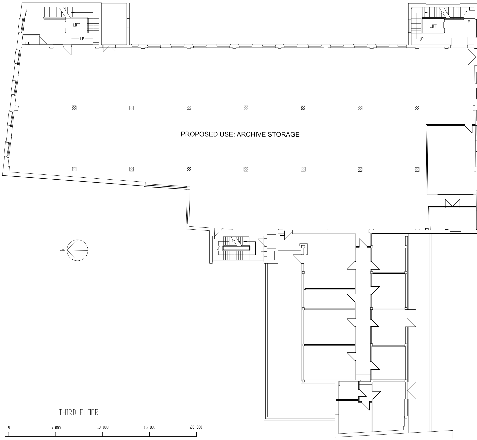
THIRD FLOOR - GA PLAN PROPOSED 1:100@A1, 1:200@A3
