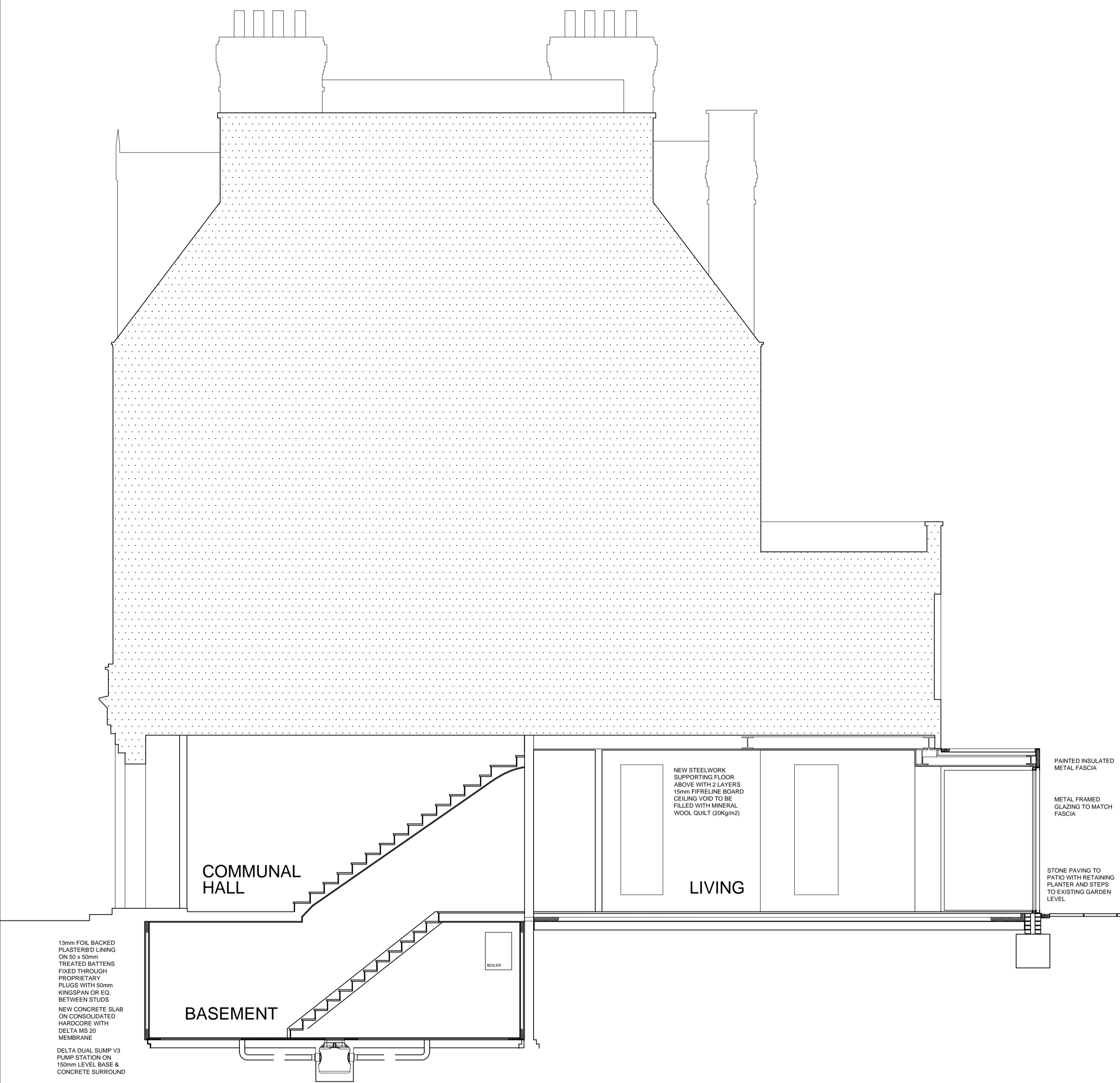
SECTION
