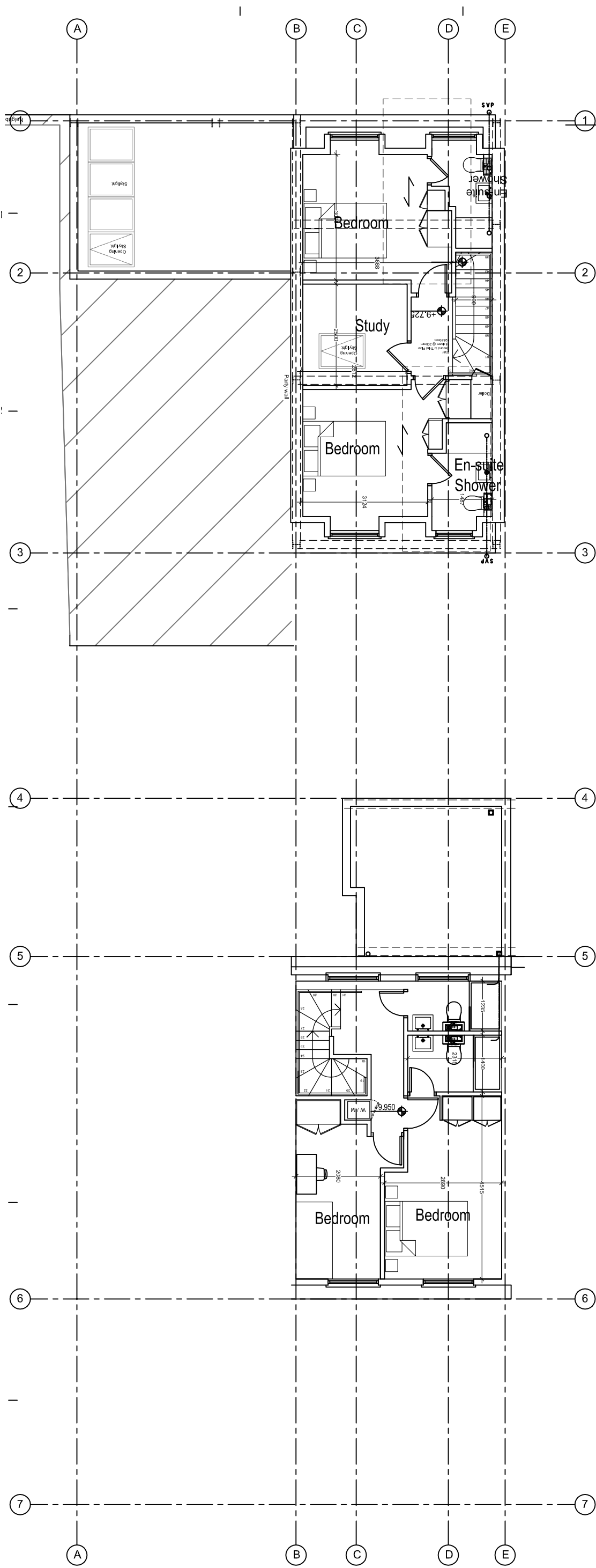
7A THIRD FLOOR PLAN SCALE 1:100
