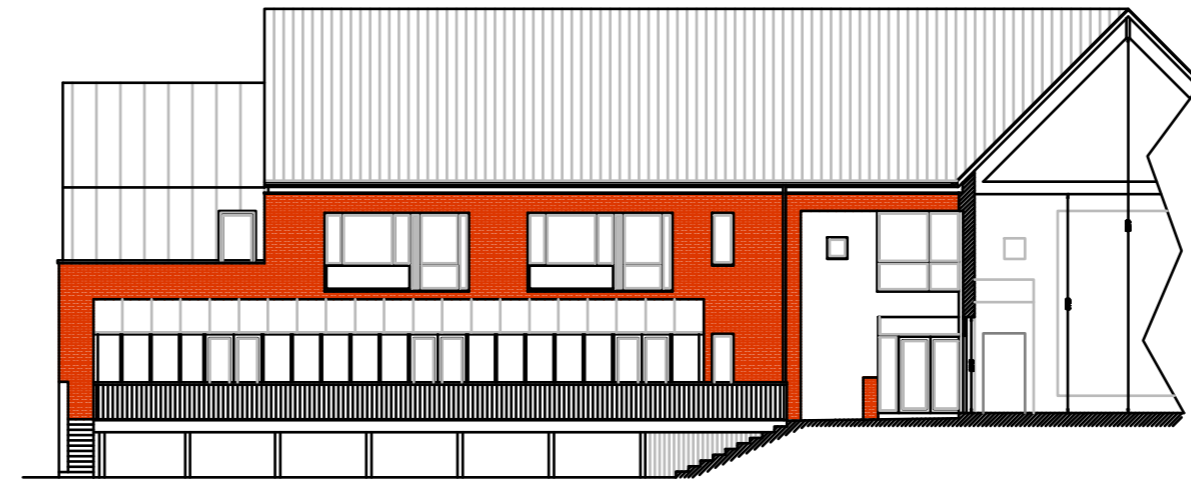
Section - Elevation 5
