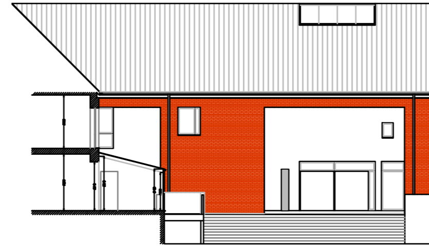
Section - Elevation 2
