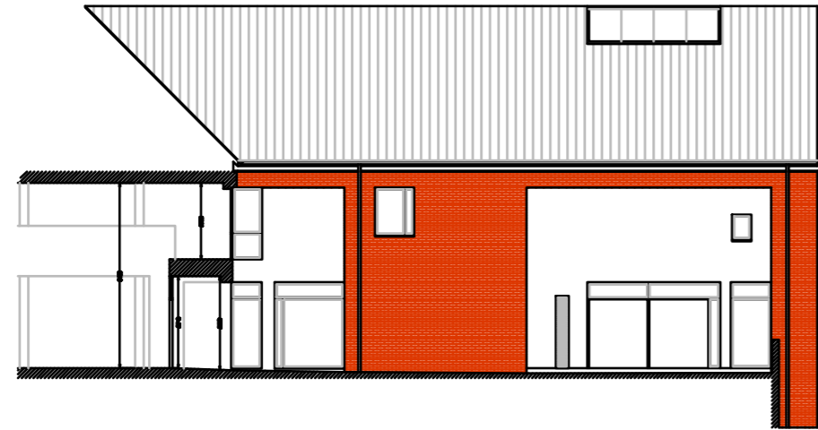
Section - Elevation 1
