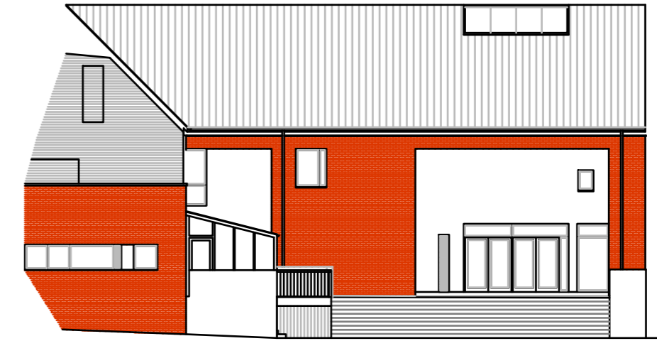
Section - Elevation 3
