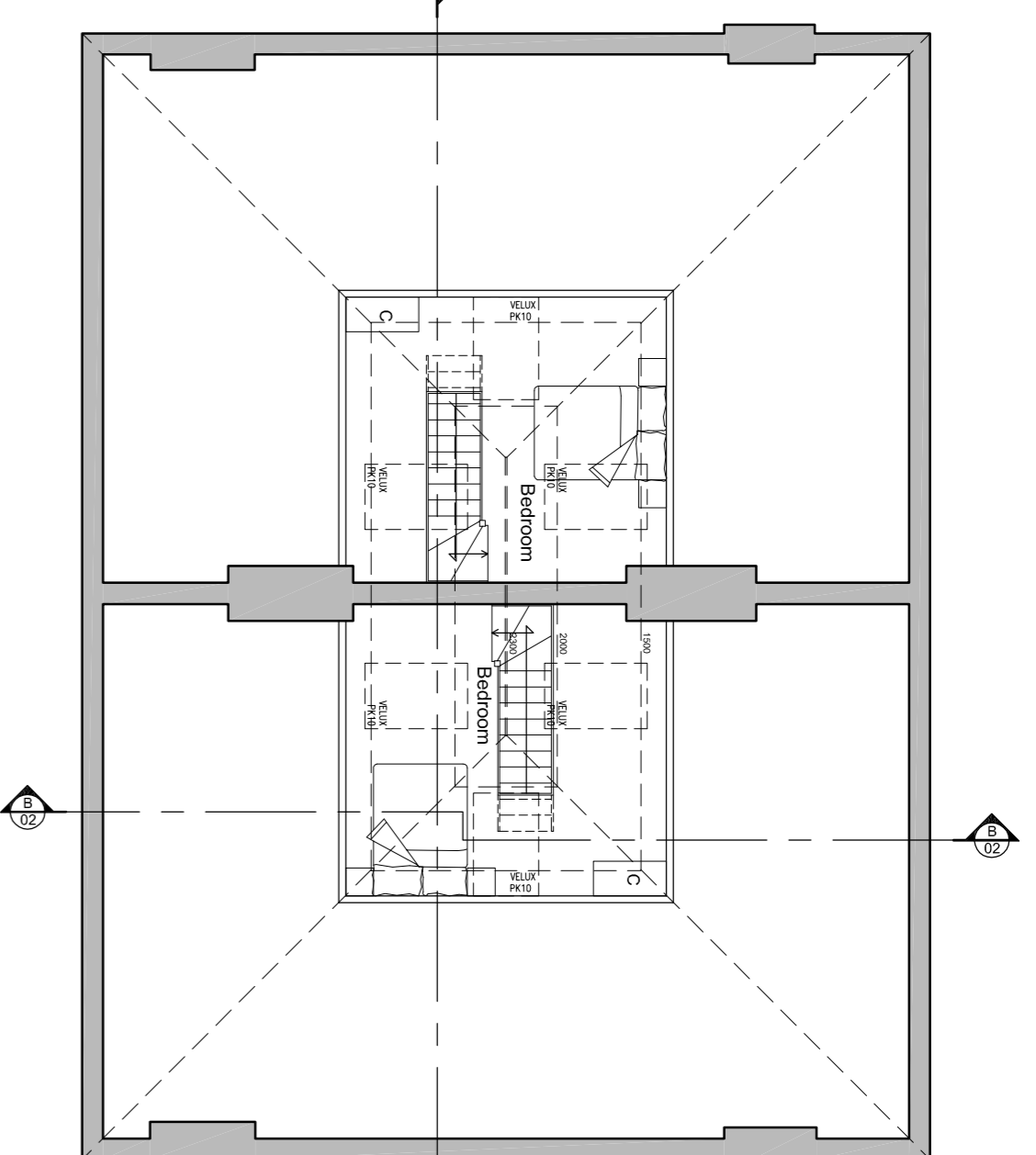
Attic Floor Plan Scale - 1:100
