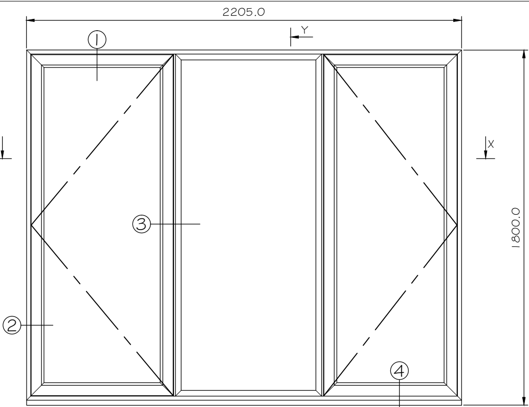
PROPOSED SIDE HUNG ALUMINIUM WINDOW 16No. REQ'D VIEWED EXTERNALLY FINISHED WHITE
