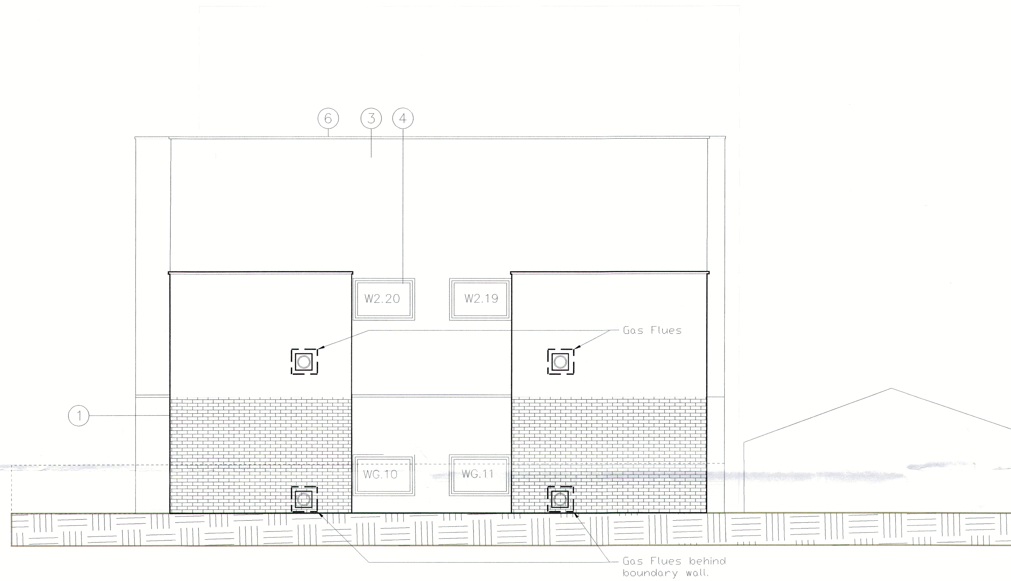
Rear Elevation
