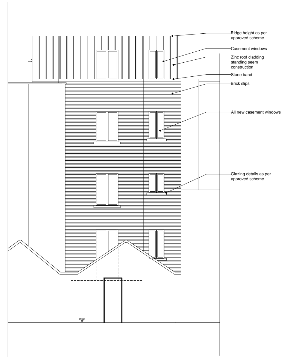
REAR ELEVATION
