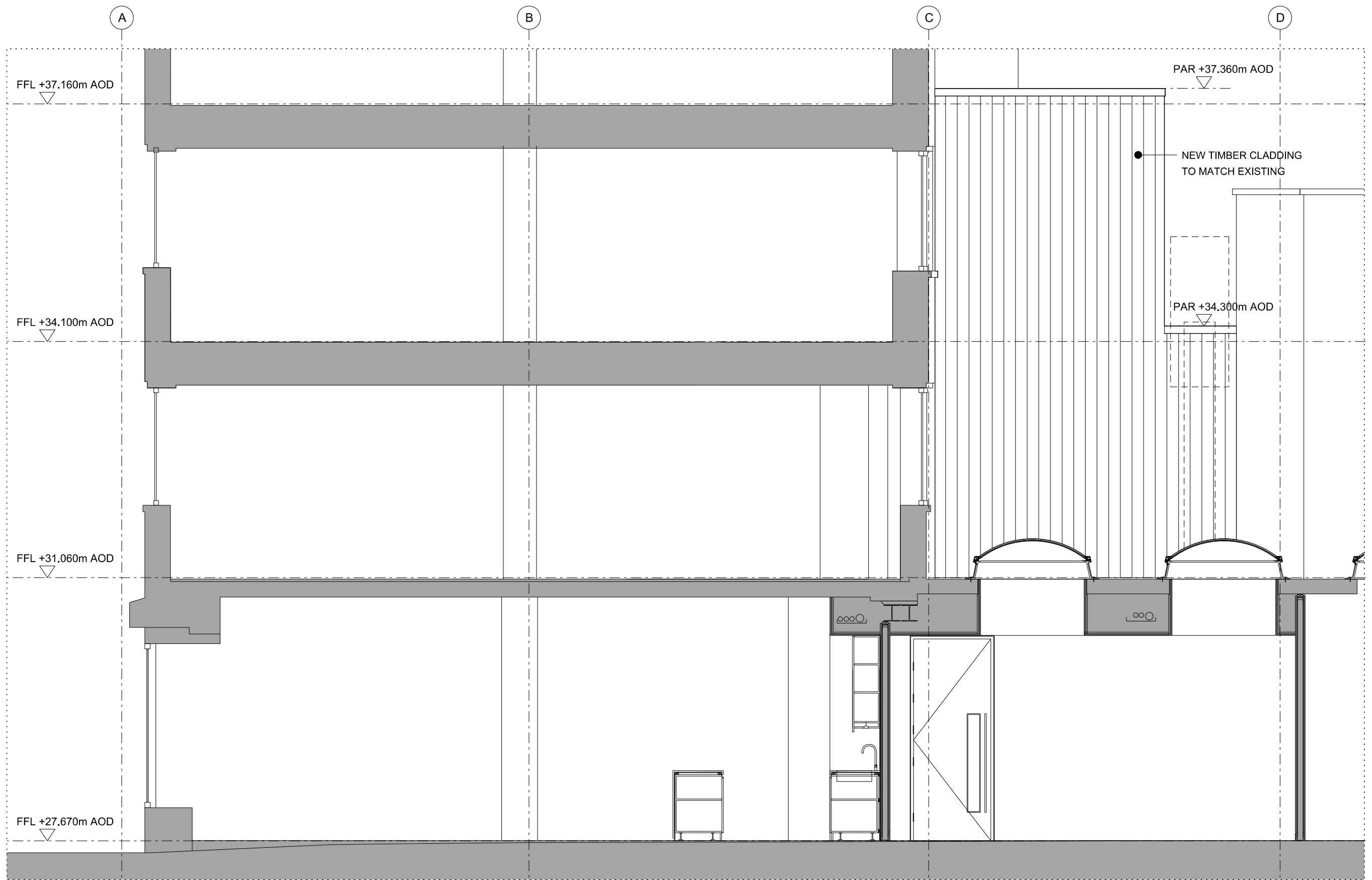
PROPOSED EAST ELEVATION/ SECTION
