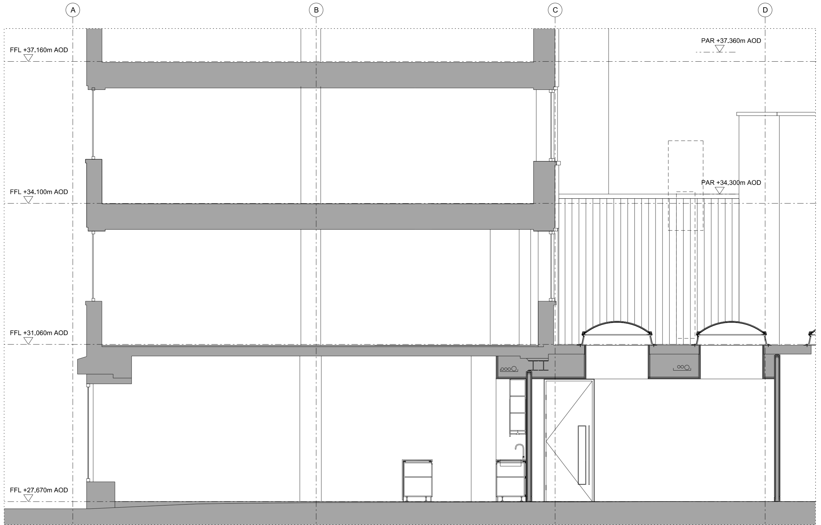
EXISTING EAST ELEVATION/ SECTION
