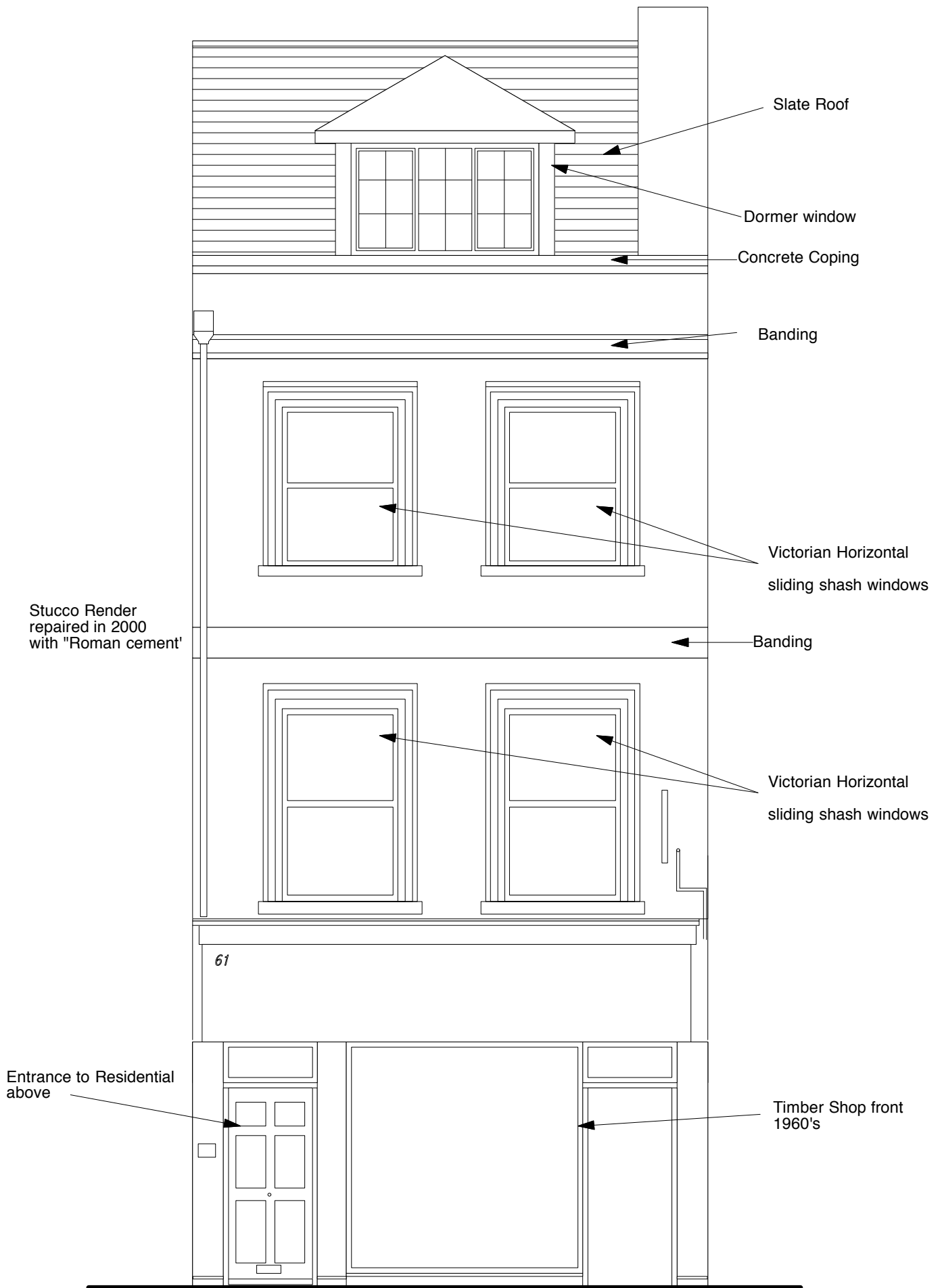
FRONT ELEVATION
