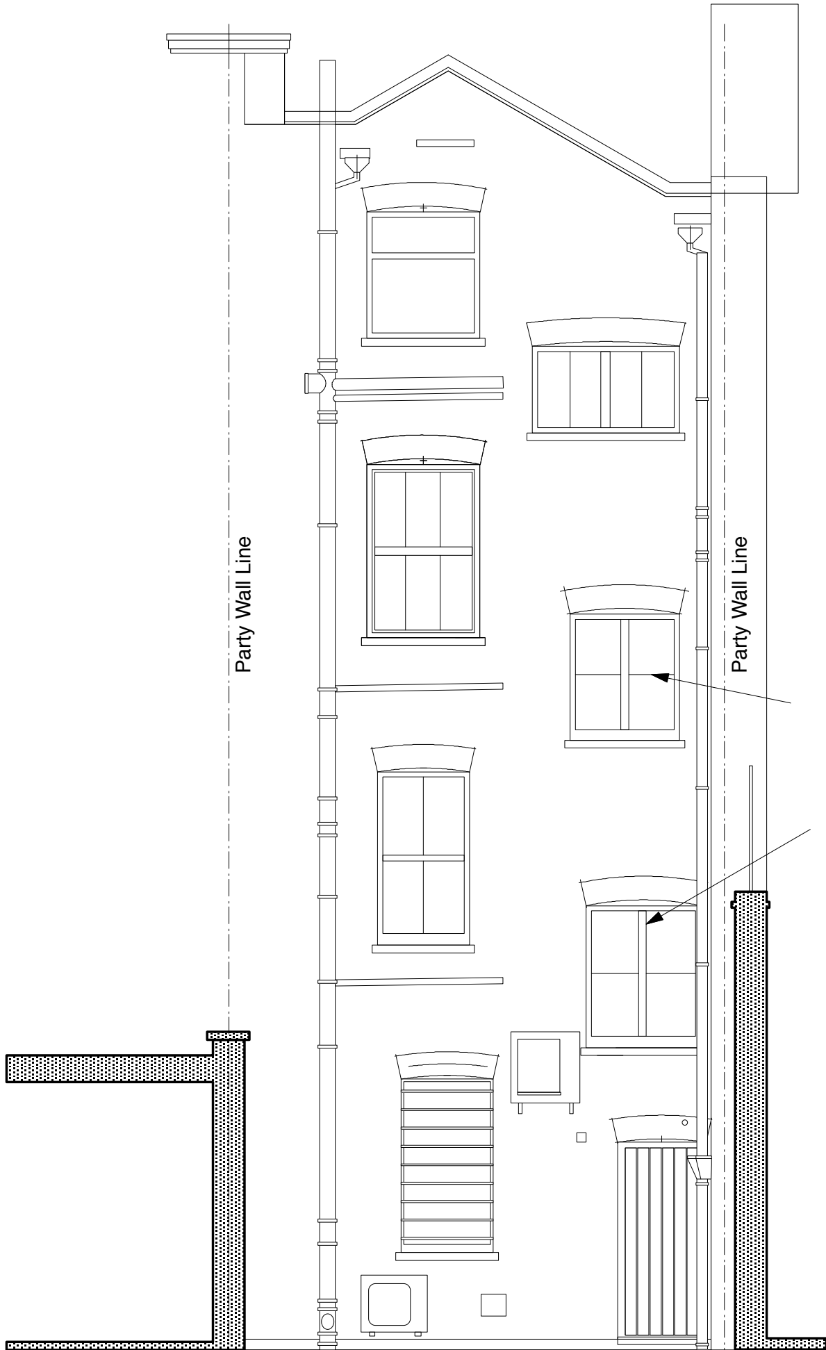
REAR ELEVATION
