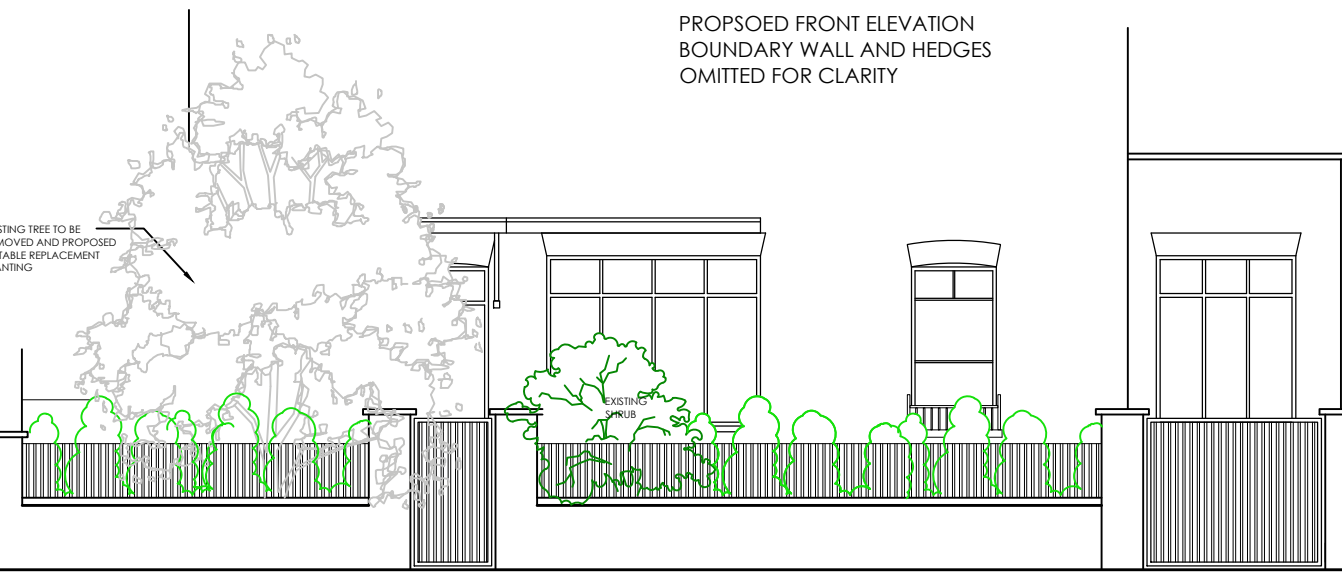
PROPOSED FRONT ELEVATION FROM PAVEMENT
