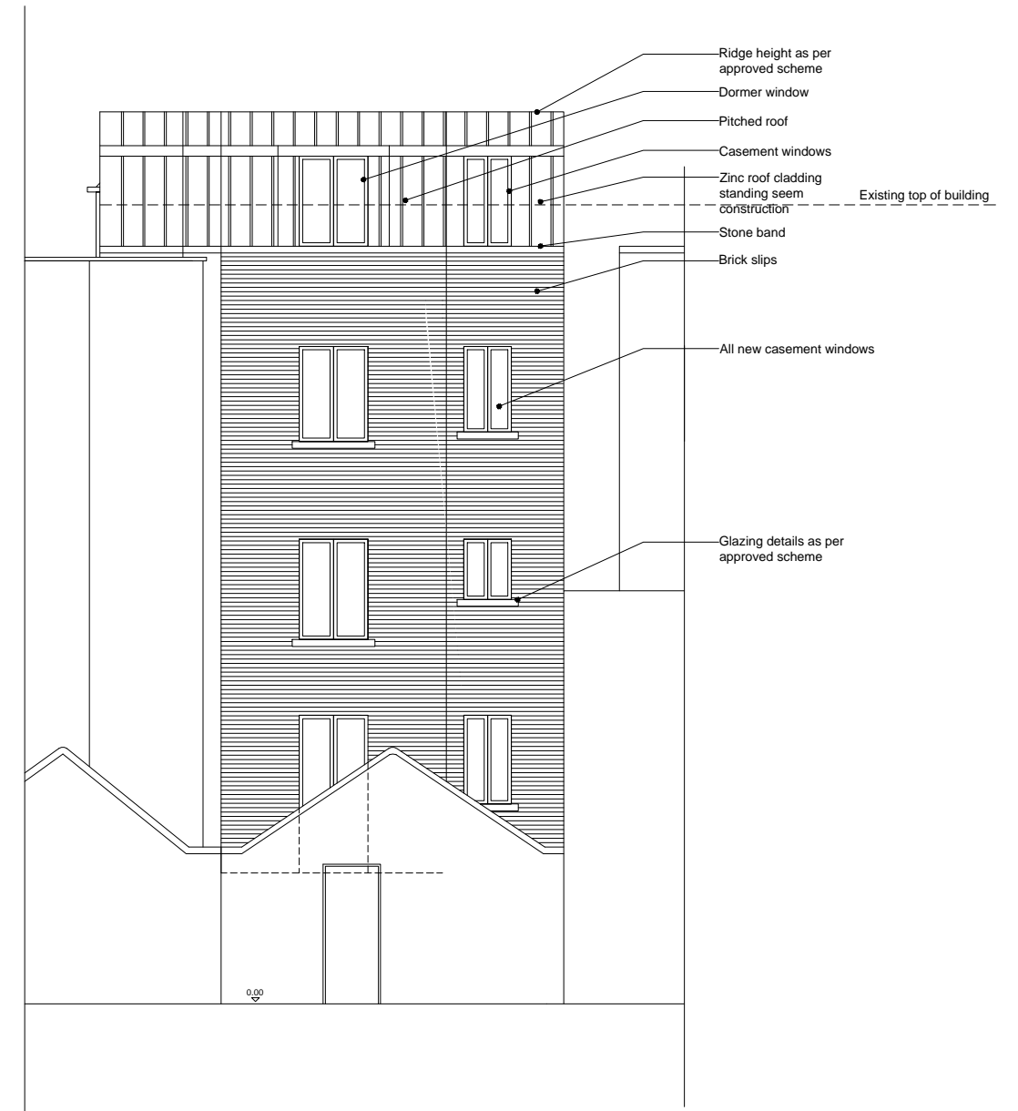
REAR ELEVATION
