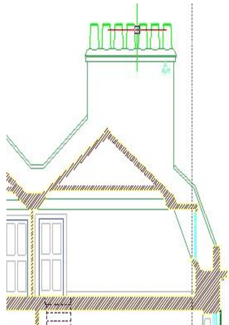
8. Typical section showing front stack. Note the stack projects beyond the ridgeline.
