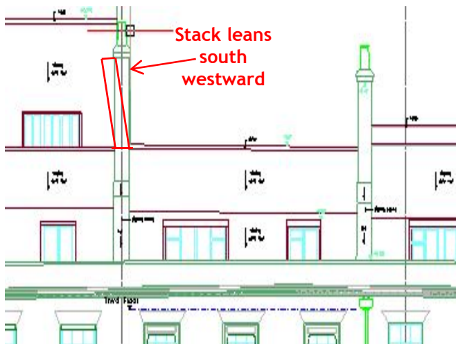
7. Part front elevation.
