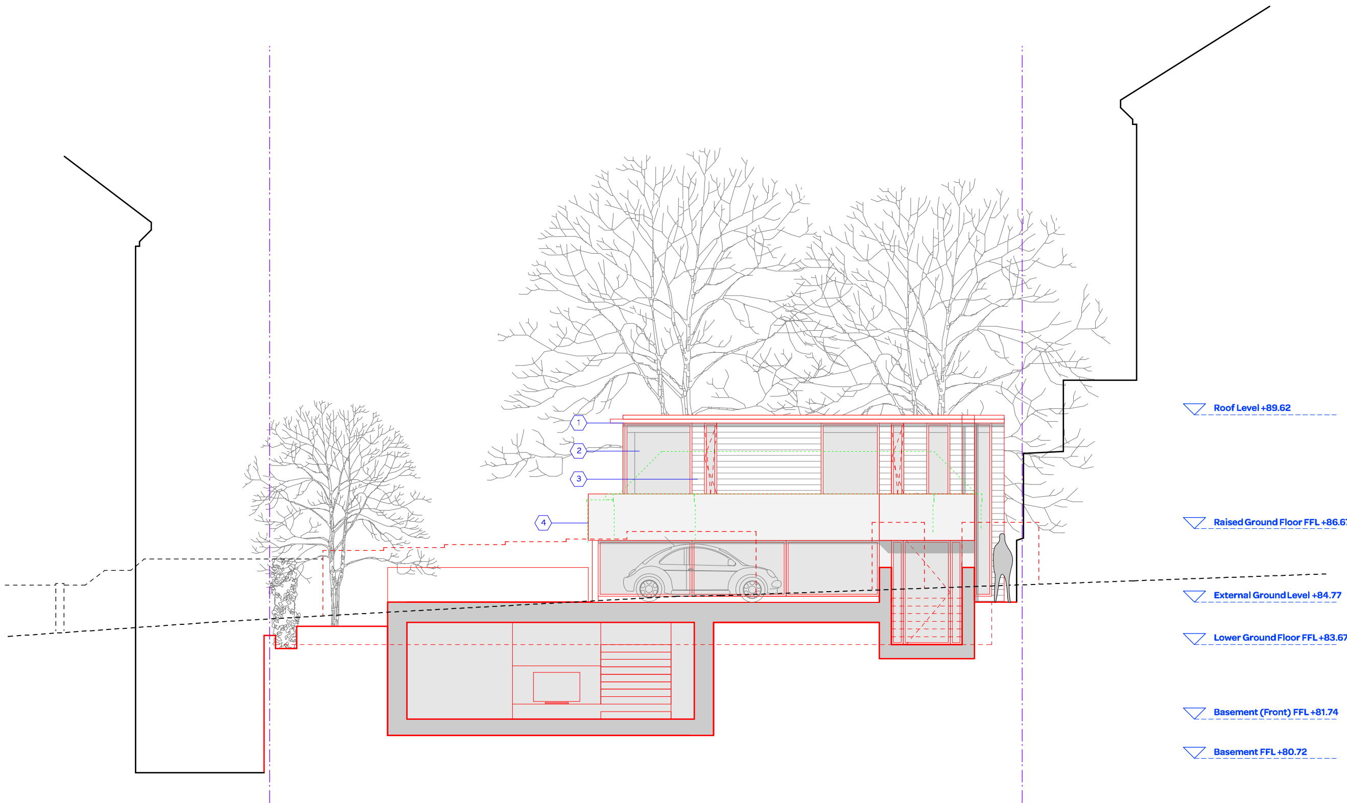
PROPOSED FRONT ELEVATION / SECTION CC
