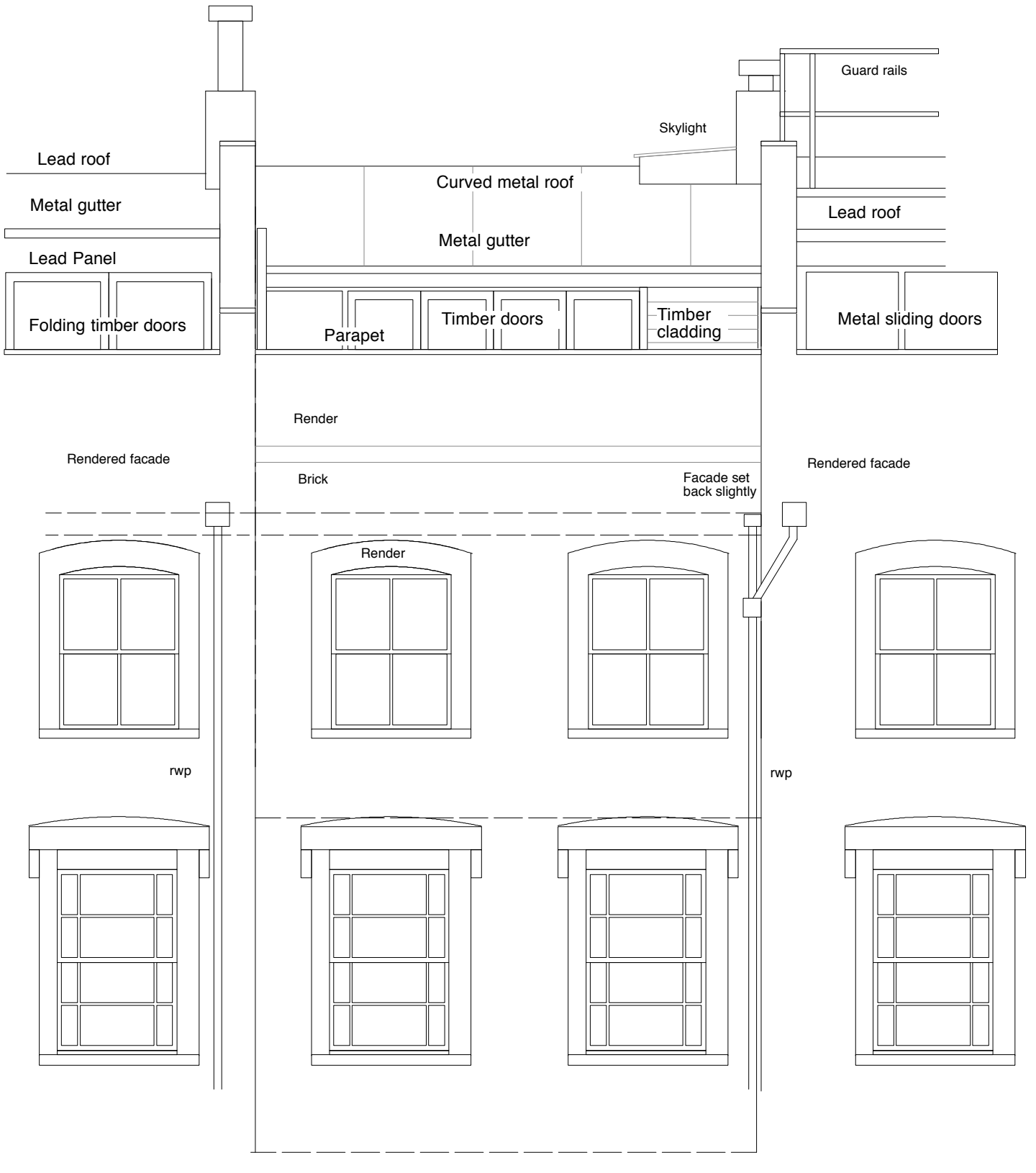
Front (East) Elevation
