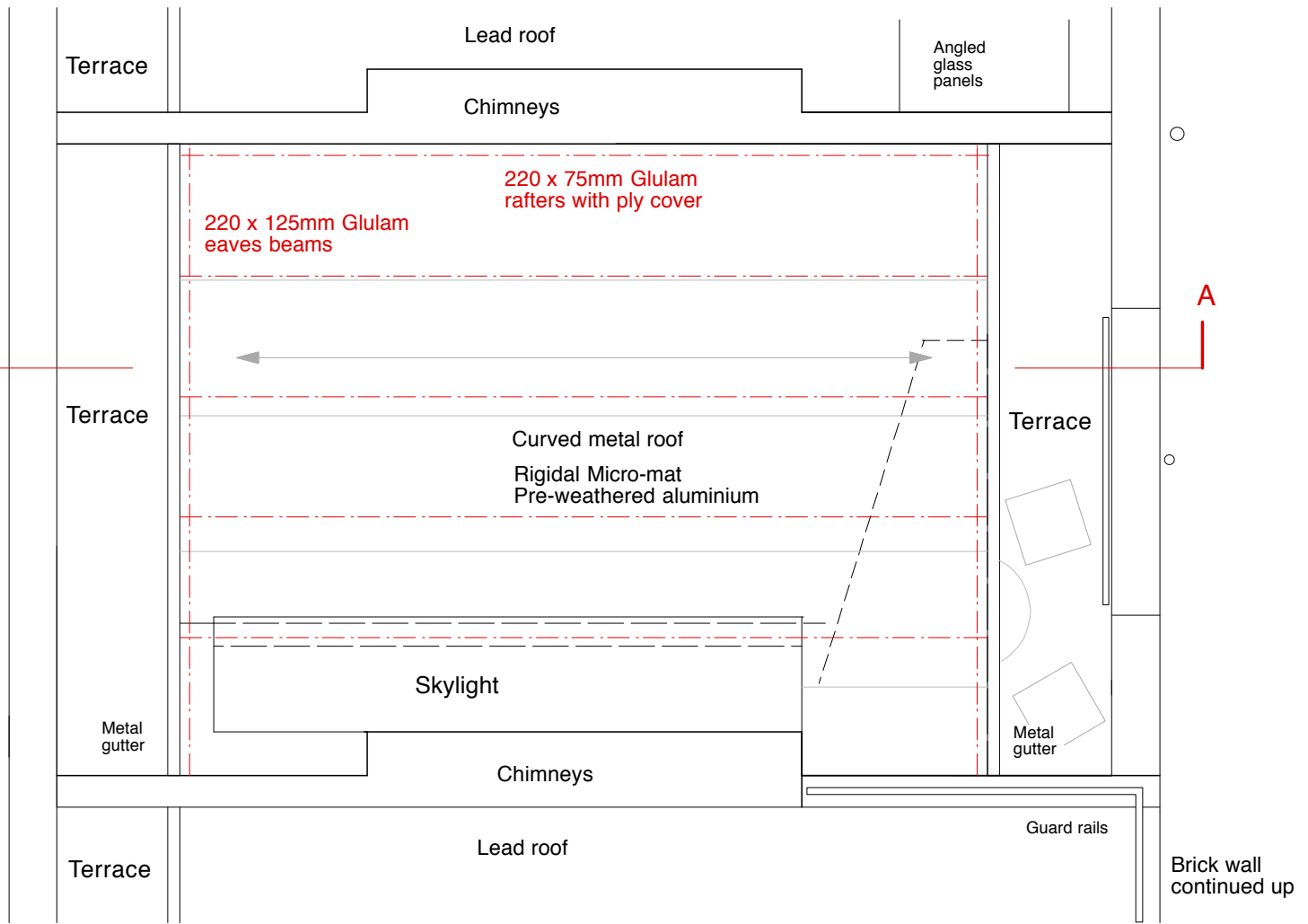
Roof Plan
