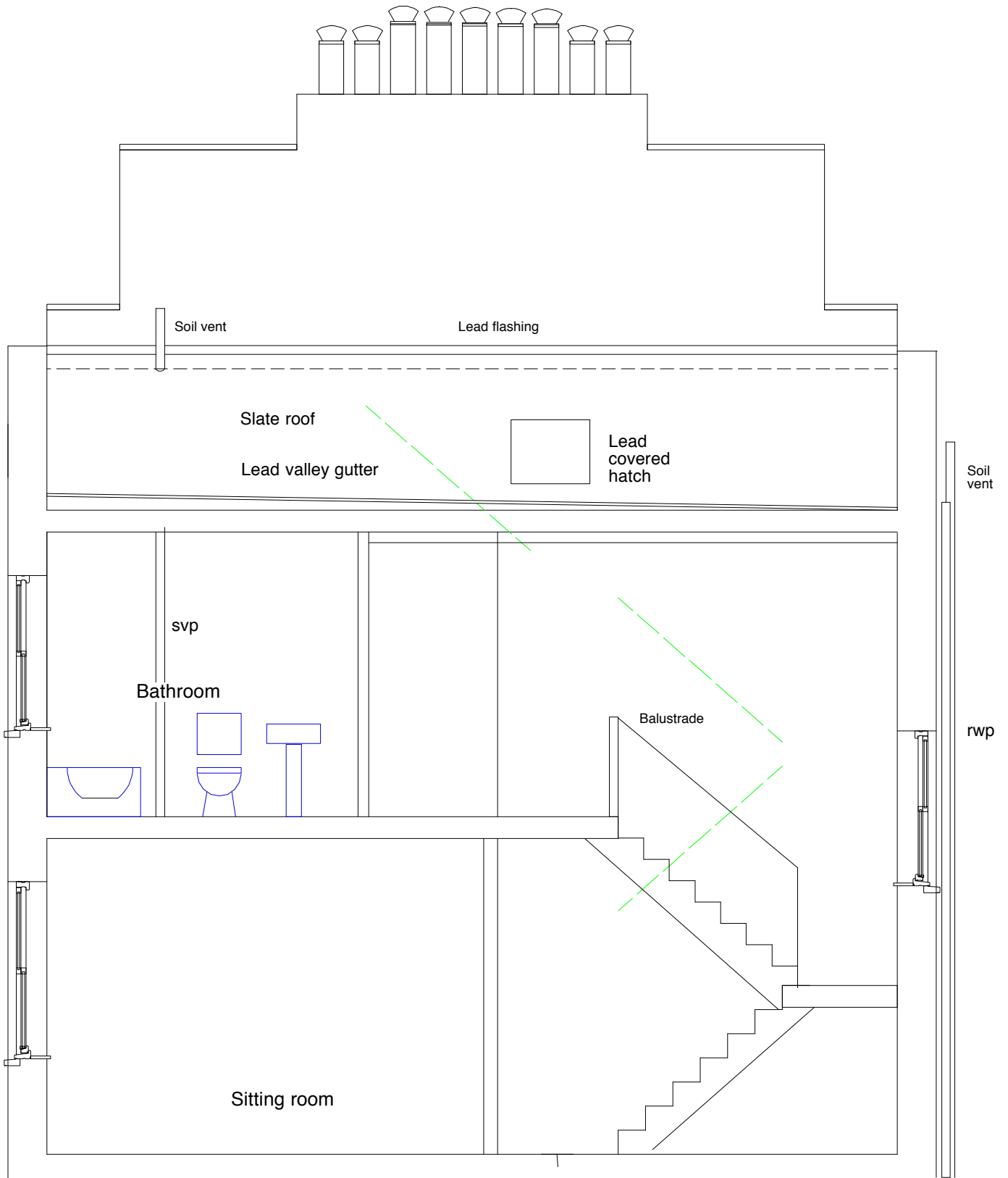
Existing Section AA
