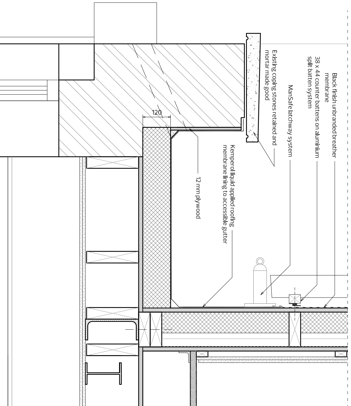
DETAIL 3 - Section at existing West parapet level
