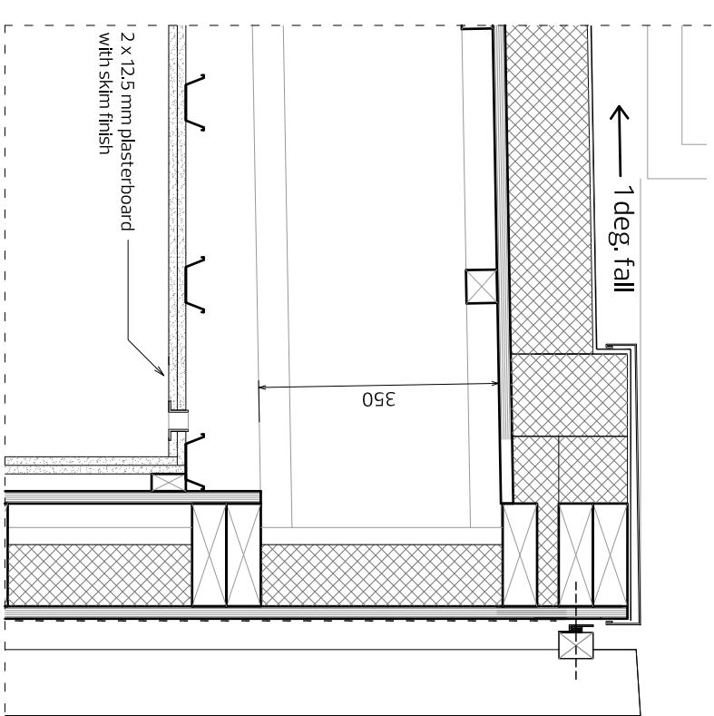
DETAIL 2 - Section at roof extension East parapet level
