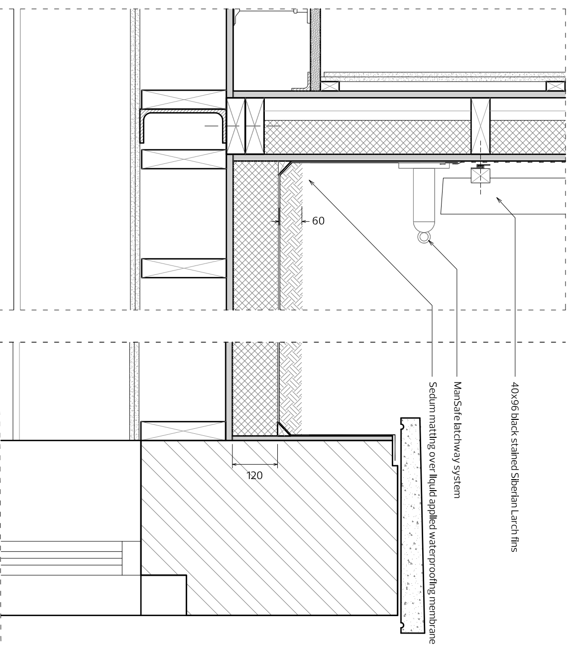
DETAIL 4 & 5 - Section at existing East parapet level
