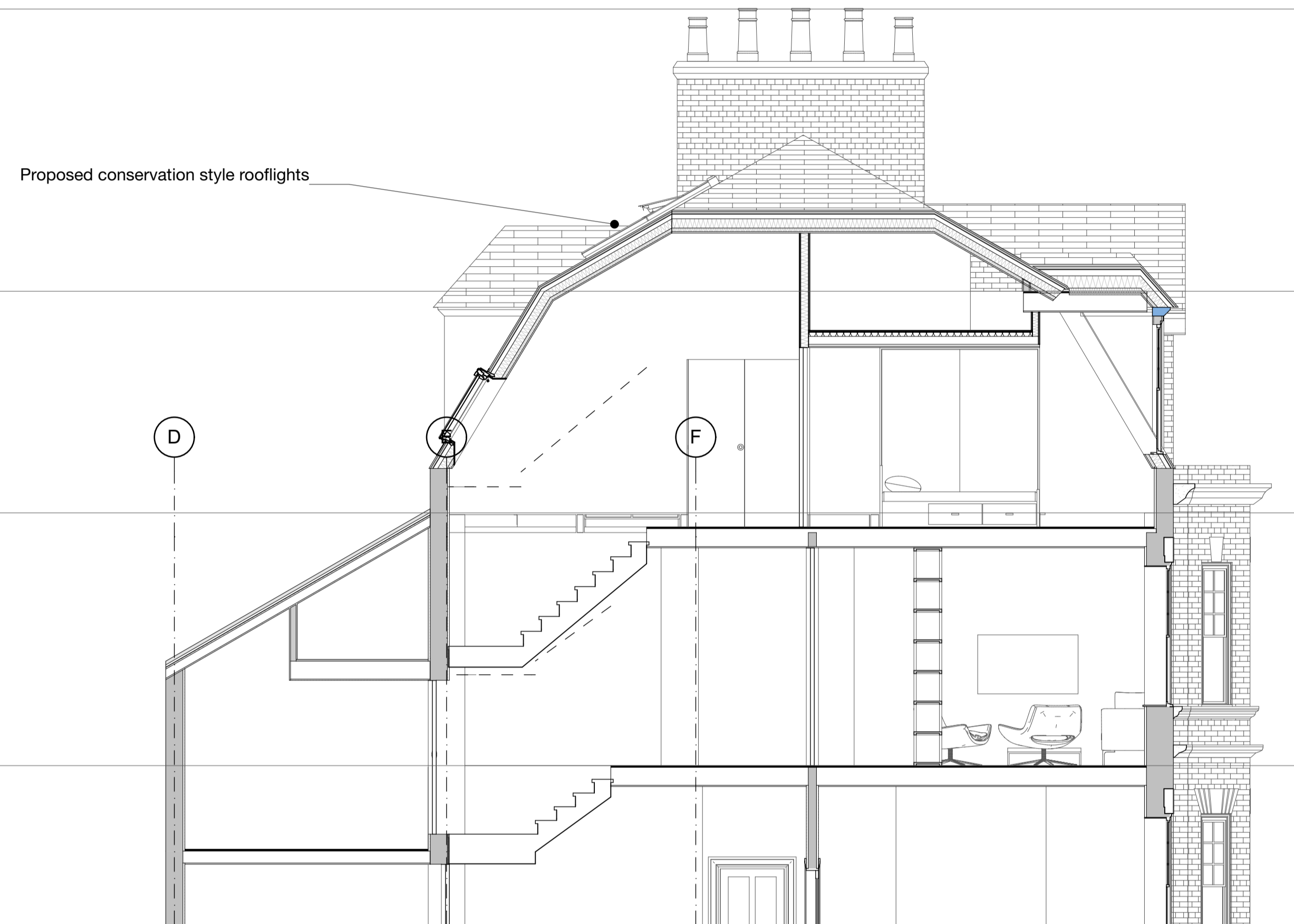
Section C-C as Existing 1:50
