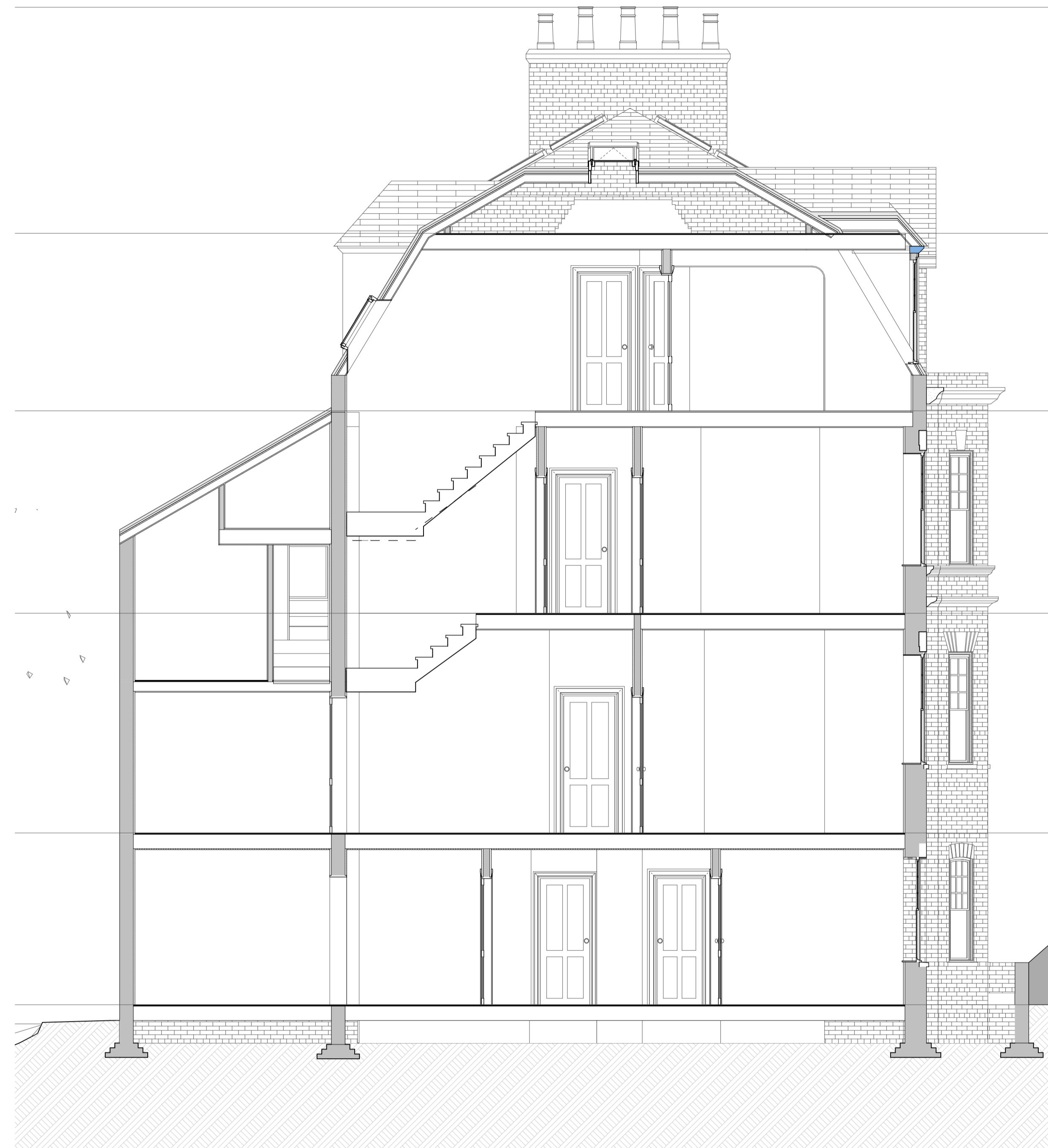
Part Section C-C as proposed 1:50
