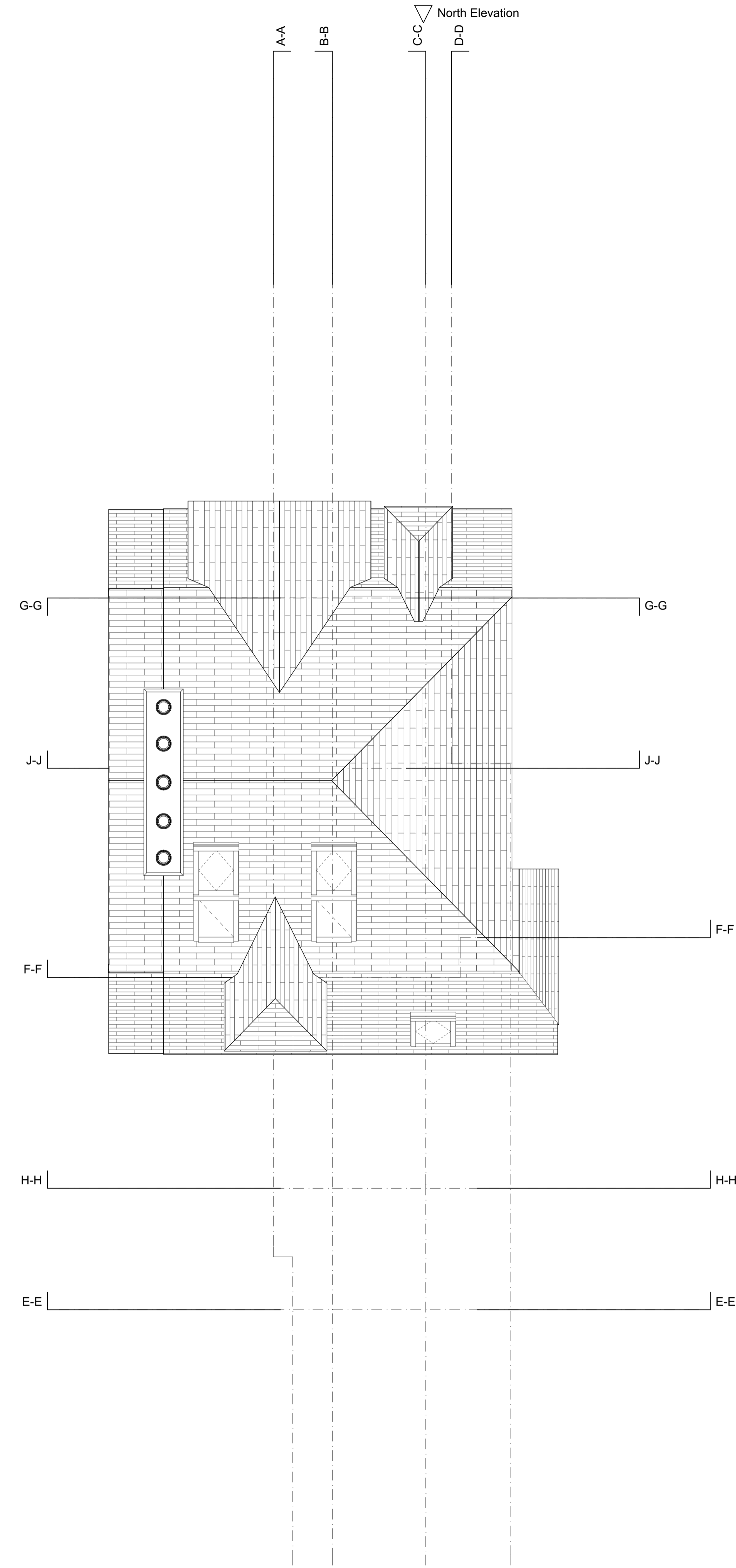
Roof Proposed 1:50
