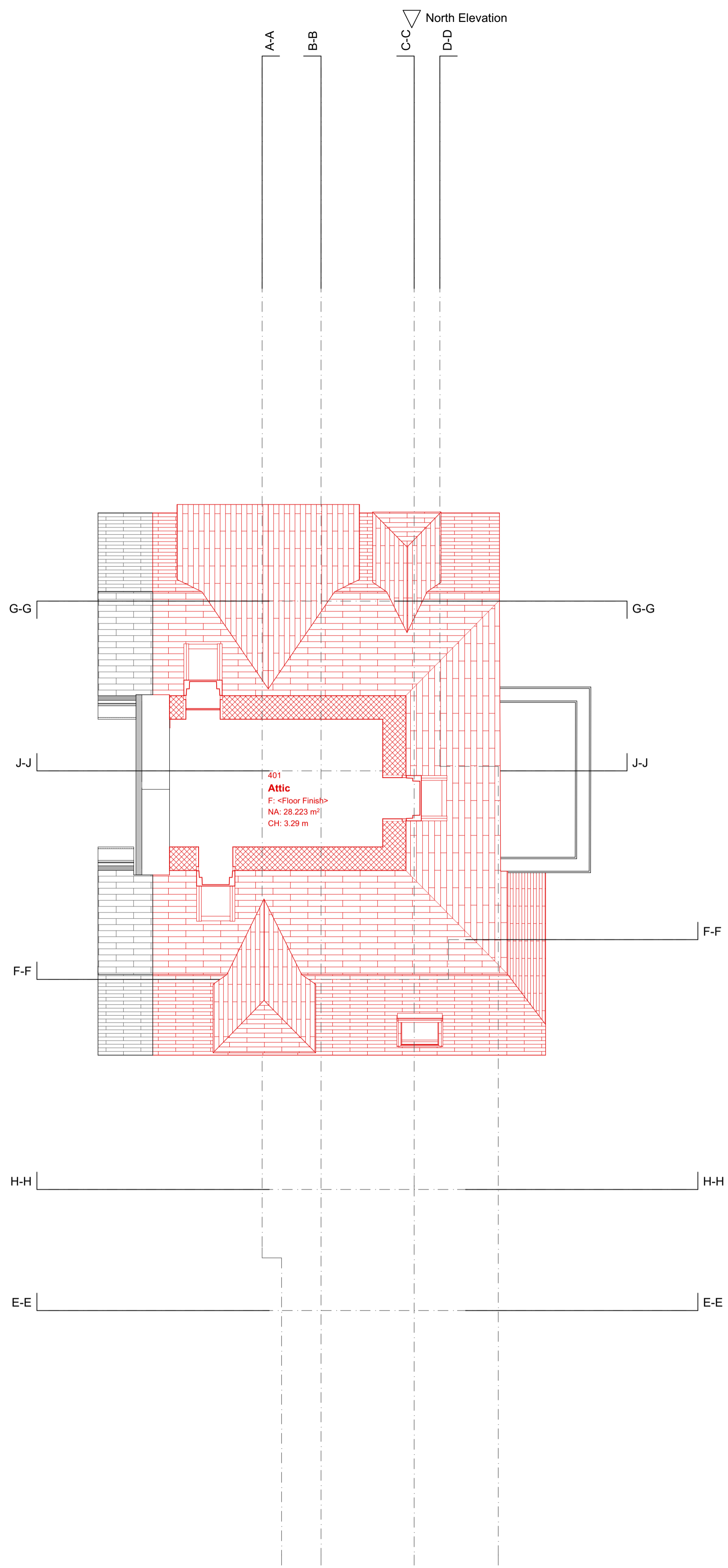
Attic Floor Demolitions 1:50
