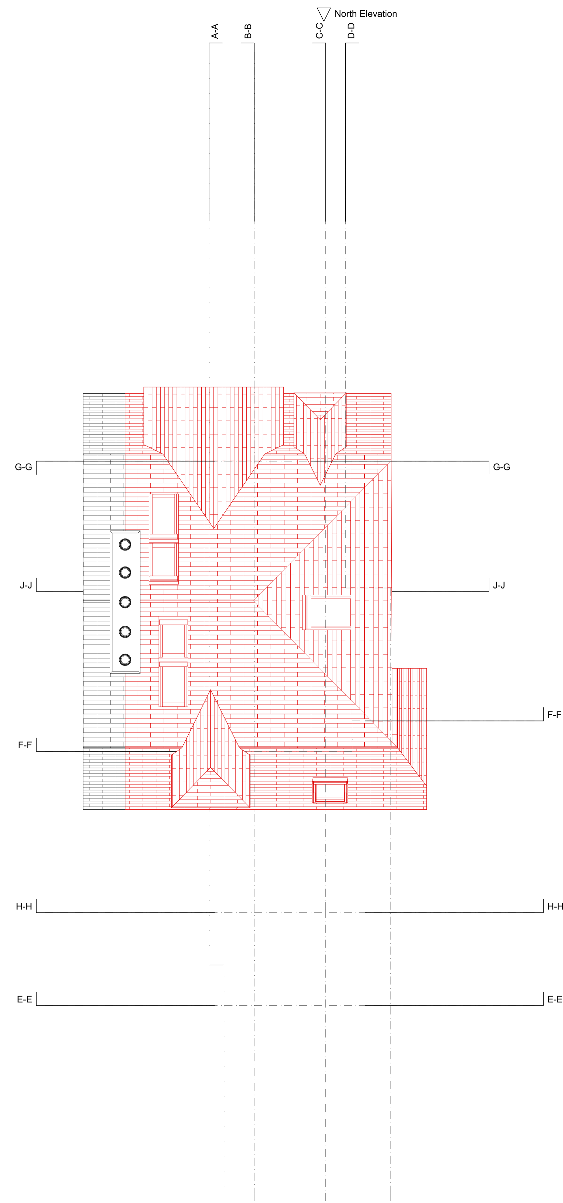
Roof Demolitions 1:50
