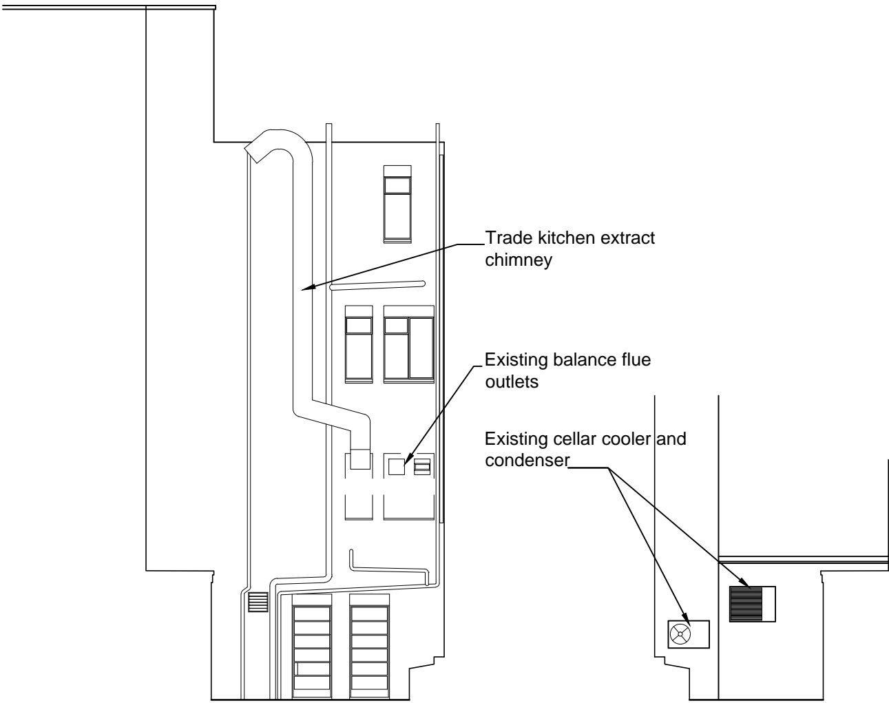
Elevation A (existing) scale 1:100 @ A1 Elevation B (existing) scale 1:100 @ A1
