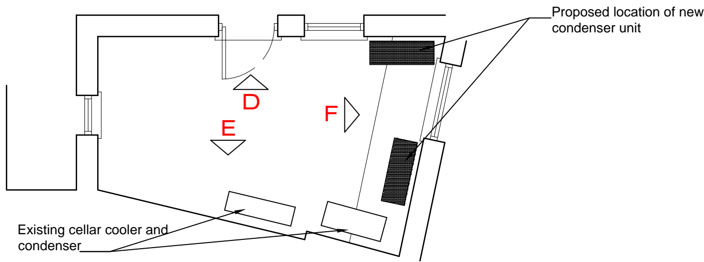
Rear Yard Layout (proposed) scale 1:50 @ A1
