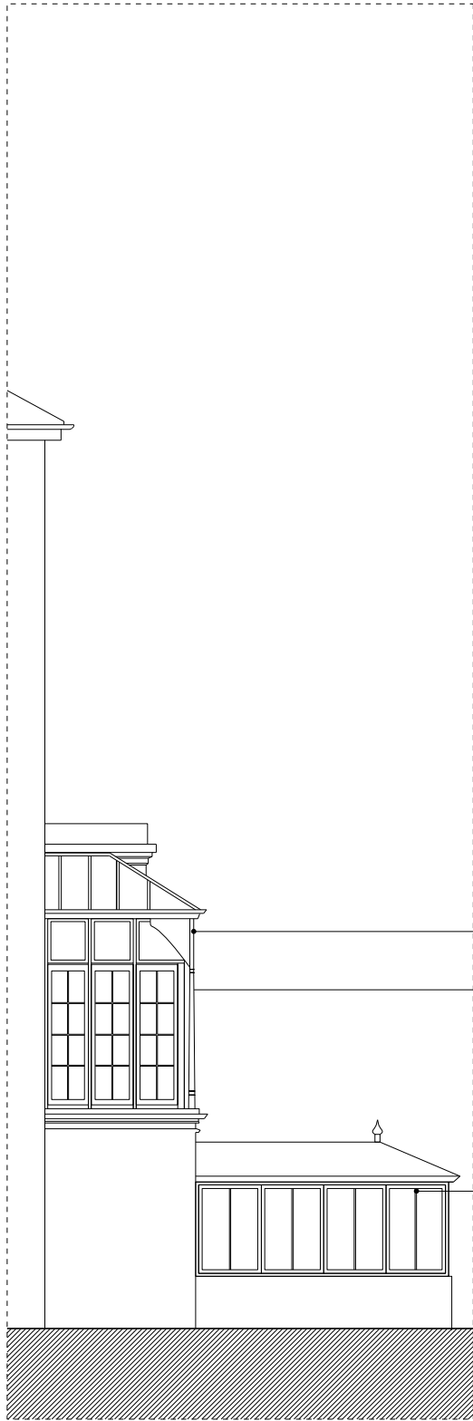
01 EXISTING ELEVATION AA 02-100 1:100 @ A3
