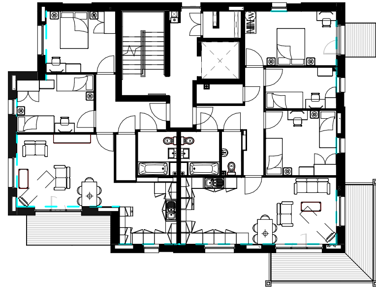
BLOCK F FIFTH FLOOR PLAN Approved Under Application ref 2013/1924/P
