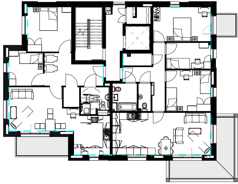
BLOCK F SECOND FLOOR PLAN Approved Under Application ref 2013/1924/P
