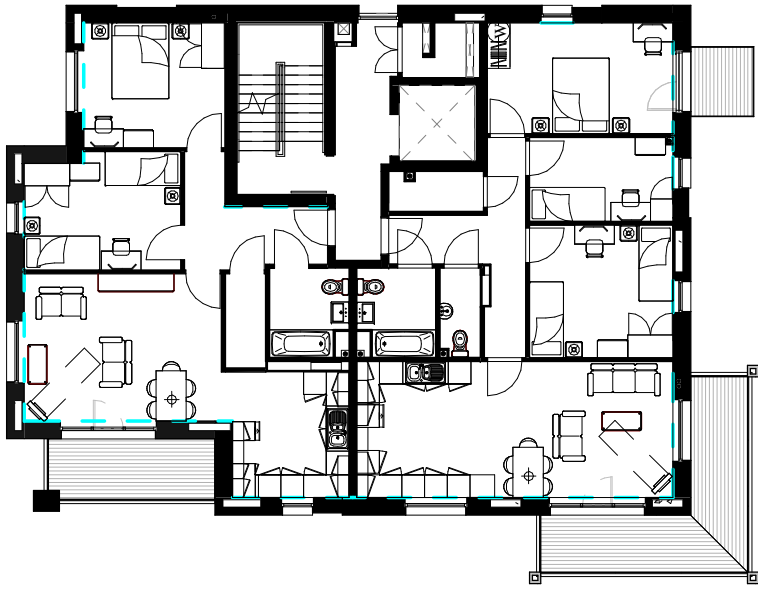
BLOCK F FOURTH FLOOR PLAN Approved Under Application ref 2013/1924/P
