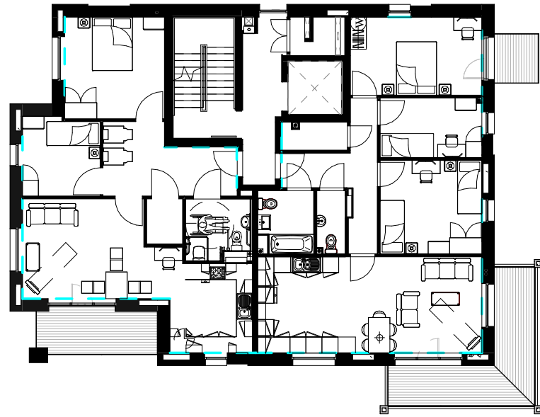
BLOCK F THIRD FLOOR PLAN Approved Under Application ref 2013/1924/P
