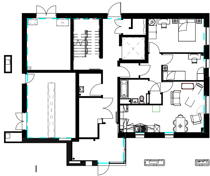
BLOCK F GROUND FLOOR PLAN Approved Under Application ref 2013/1924/P
