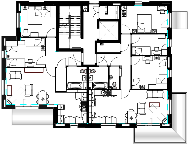
BLOCK F SIXTH FLOOR PLAN Approved Under Application ref 2013/1924/P
