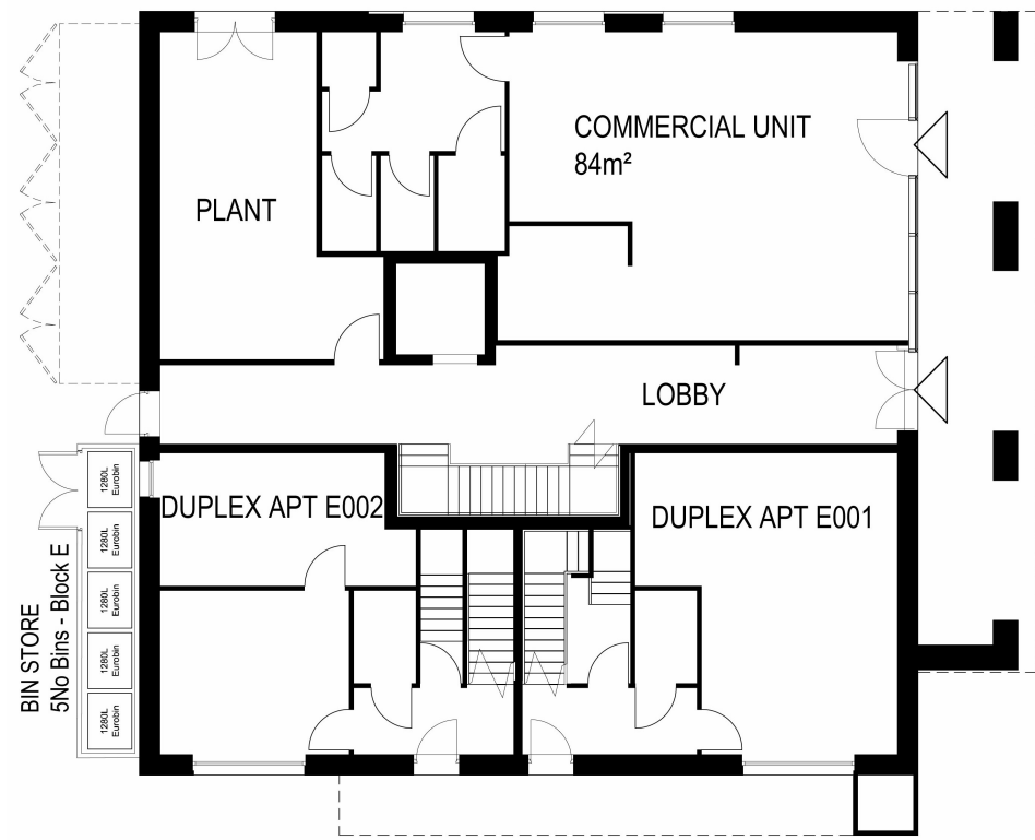
BLOCK E GROUND FLOOR PLAN Approved Under Application Ref 2013/6627/P
