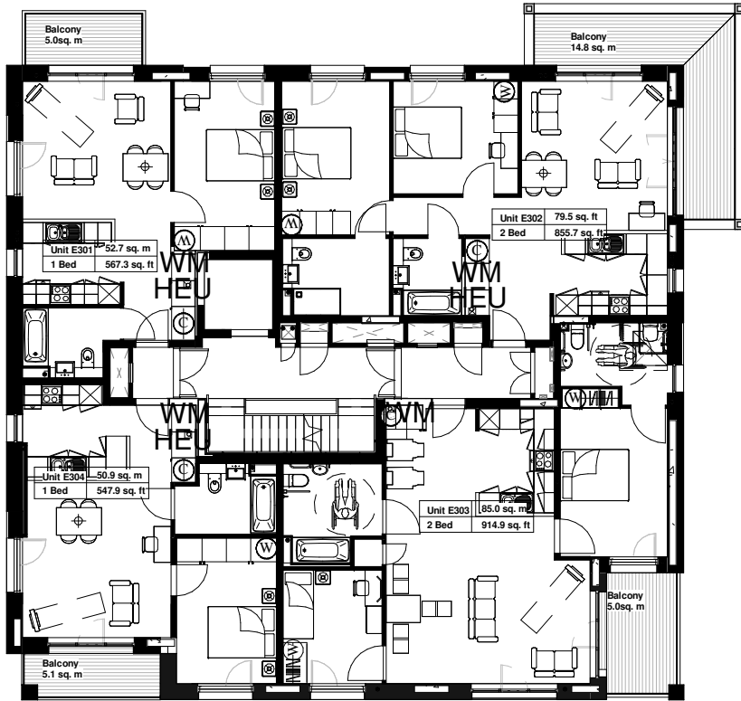
BLOCK E THIRD FLOOR PLAN Approved Under Application Ref 2013/1924/P
