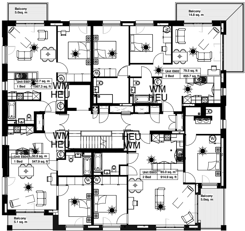
BLOCK E SIXTH FLOOR PLAN Approved Under Application Ref 2013/1924/P
