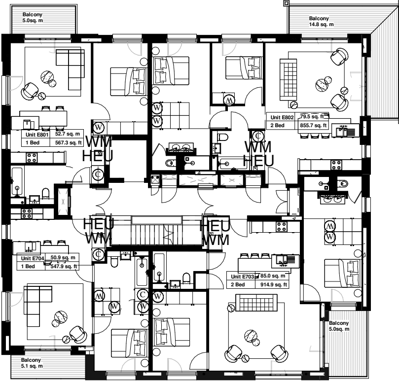
BLOCK E EIGHTH FLOOR PLAN Approved Under Application Ref 2013/1924/P
