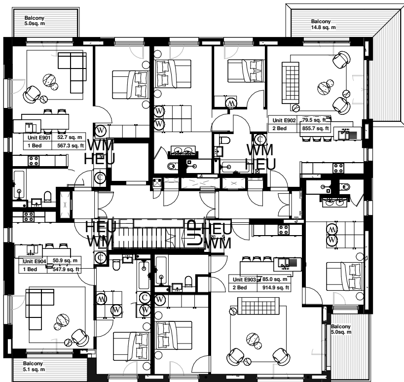
BLOCK E NINTH FLOOR PLAN Approved Under Application Ref 2013/1924/P
