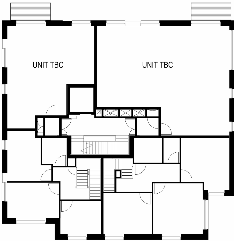
BLOCK E FIRST FLOOR PLAN Approved Under Application Ref 2014/5816/P
