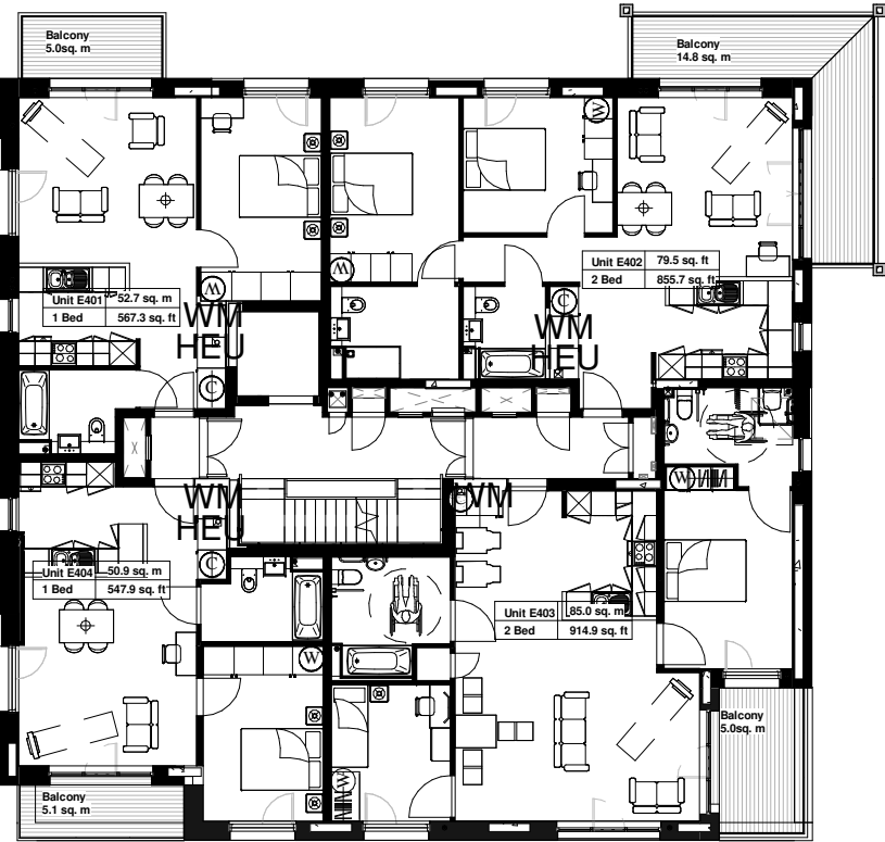
BLOCK E FOURTH FLOOR PLAN Approved Under Application Ref 2013/1924/P
