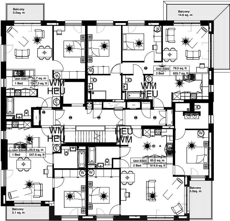
BLOCK E SECOND FLOOR PLAN Approved Under Application Ref 2013/1924/P
