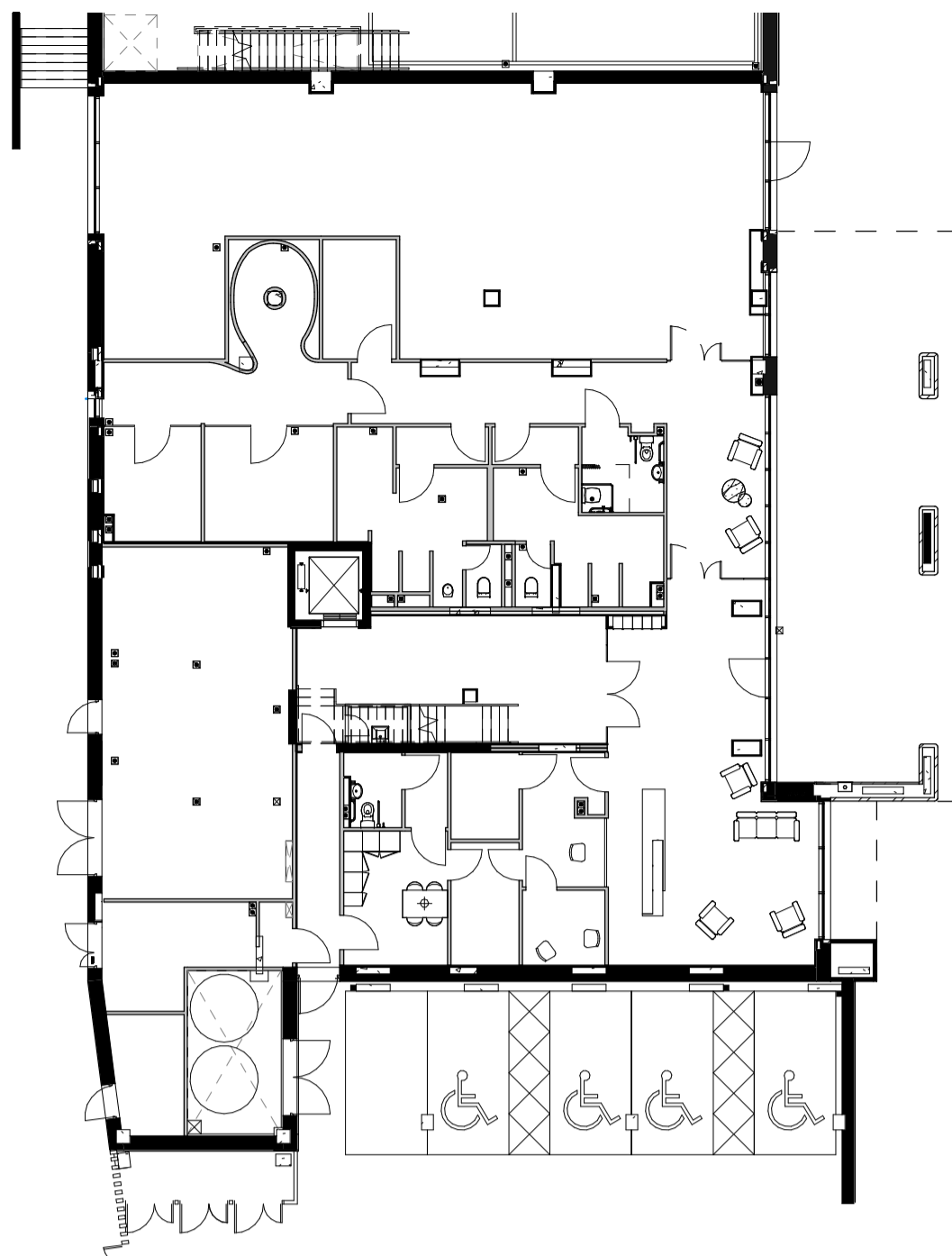
BLOCK B GROUND FLOOR PLAN
