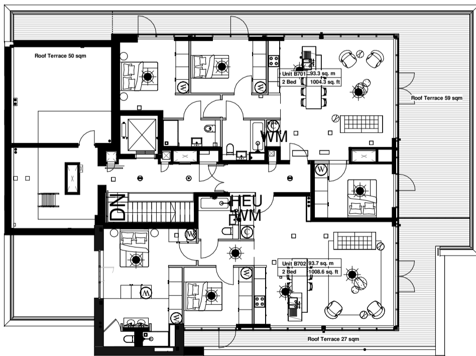
BLOCK B SEVENTH FLOOR PLAN
