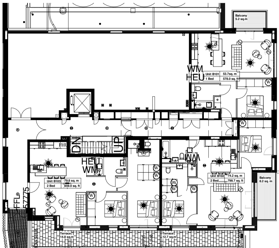
BLOCK B FIRST FLOOR PLAN Approved Under Application Ref 2013/1924/P
