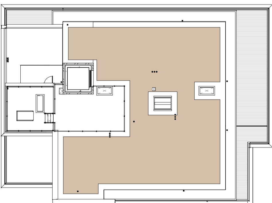
BLOCK B ROOF PLAN
