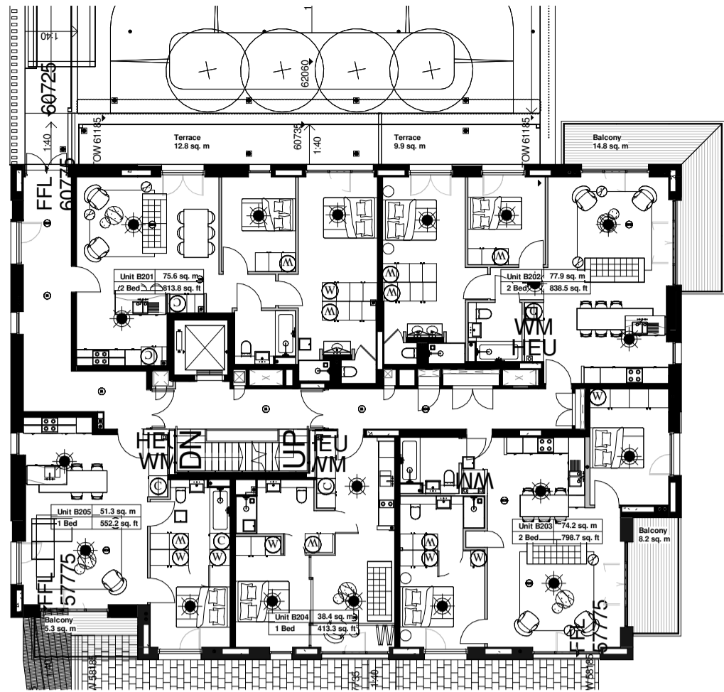
BLOCK B SECOND FLOOR PLAN Approved Under Application Ref 2013/1924/P
