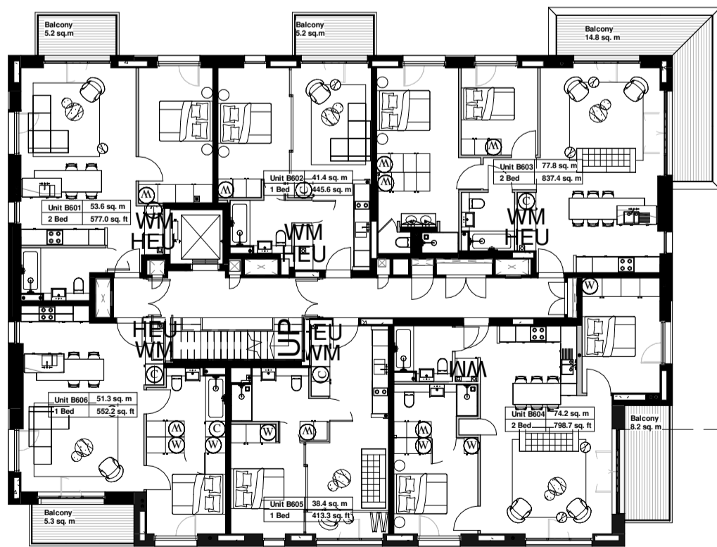
BLOCK B SIXTH FLOOR PLAN Approved Under Application Ref 2013/1924/P
