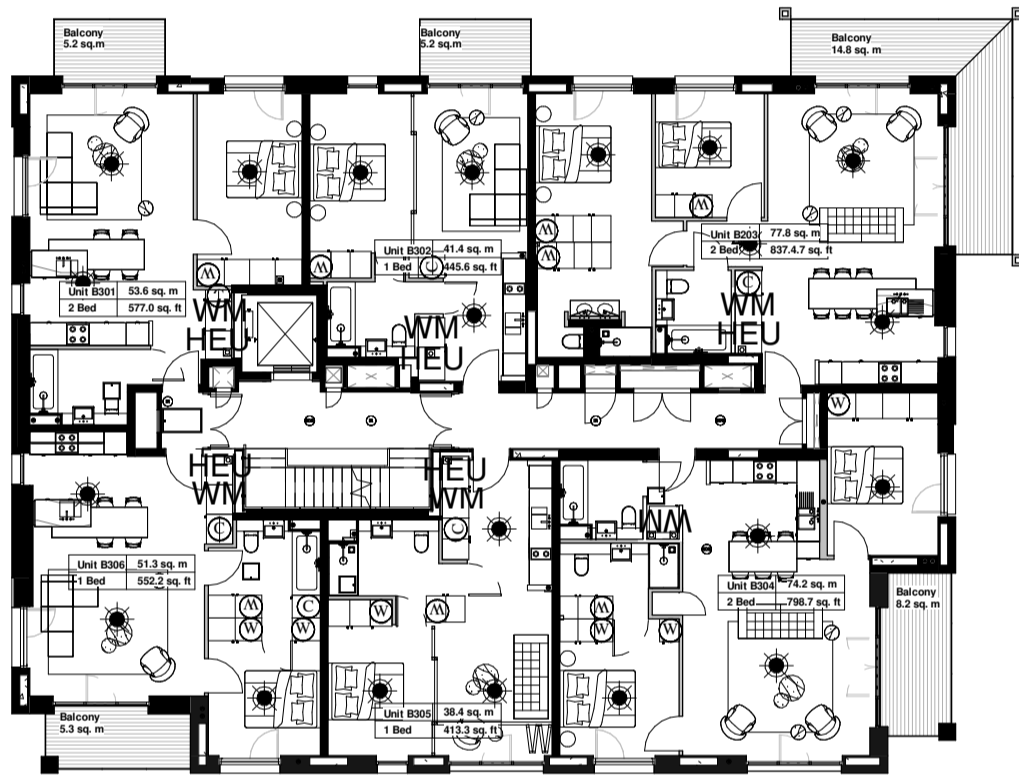
BLOCK B THIRD FLOOR PLAN Approved Under Application Ref 2013/1924/P
